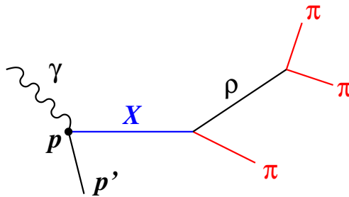
Figure 1: Decay of a resonance X into three pions via a \rho isobar.
