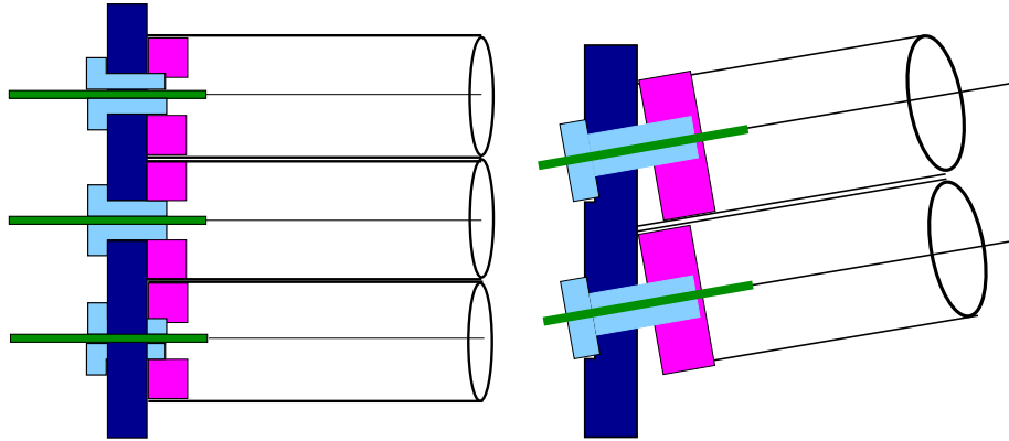
Figure 4.37: Schematic drawings of the feed throughs for both the normal ( left ) and stereo ( right ) wires.
