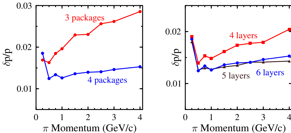
Figure 4.44: Monte Carlo studies comparing the FDC resolution in (a) a configuration with three packages vs. four packages and (b) a 4-package configuration with 4, 5, and 6 wire planes per package.
