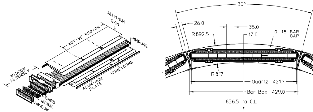
Figure 4.68: Left: View of a bar-box assembly. 12 bar-boxes surround the drift chamber. Right: Placement of the bar-box in the BABAR detector above the cylindrical drift chamber.
