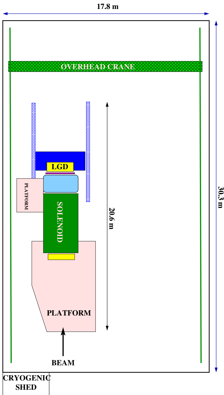
Figure 4.87: Plan view of the GLUEX experiment in HALL D.
