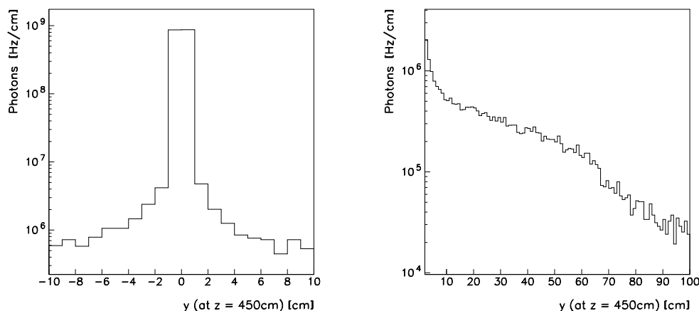
Figure 4.74: The rate of photons per cm along the y axis integrated over all of x at the location z = 450 cm. Left: rate/cm below \pm 10 cm; Right: rate/cm versus y . The innermost 3 cm are omitted.
