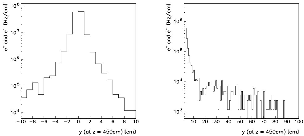
Figure 4.73: The rate of electrons and positrons per cm along the y -axis integrated over all of x at the location z = 450 cm. Left: rate/cm below \pm 10 cm in y . Right: rate/cm versus y . The innermost 3 cm are omitted.
