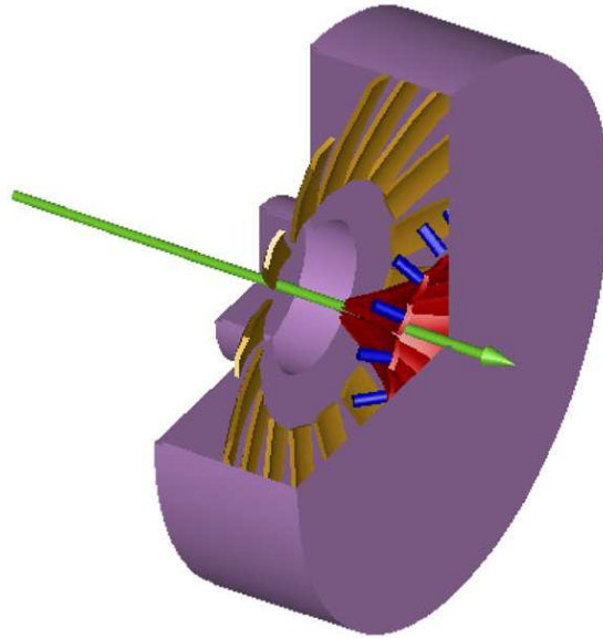
Figure 4.79: A schematic drawing of the HALL D Čerenkov detector system. The particles enter from the left into the gas volume in the center. The Čerenkov light is then reflected off the mirrors in the center (shown in dark) into the phototubes at the outer rim (shown as dark cylinders).
