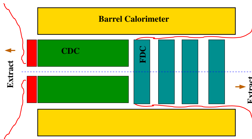
Figure 4.89: The insertion of the Central and Forward Tracking chambers inside the Barrel Calorimeter.
