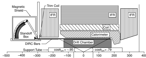
Figure 4.66: The side-view of the BABAR detector with the components of the DIRC indicated (units in cm).
