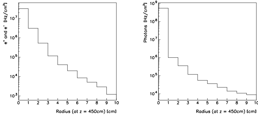
Figure 4.75: Left: The rate of electrons and positrons together per \text{cm}^2 versus radial distance from the beam axis in the virtual plane at z = 450 cm. Right: The same for photons.
