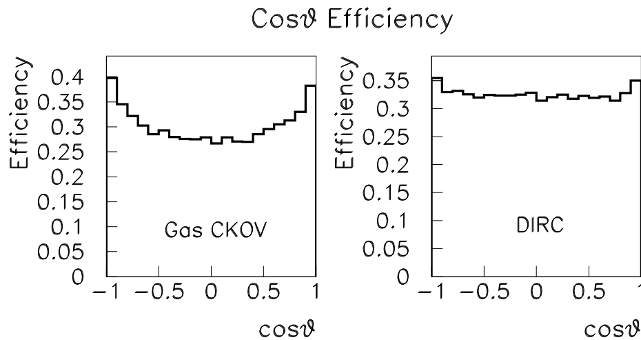
Figure 4.85: Angular efficiencies for \cos\theta in the Gottfried-Jackson coordinate system for \gamma p \rightarrow K^* \bar{K}^* p events. The left plot is for the Cerenkov option, the right for the DIRC option.
