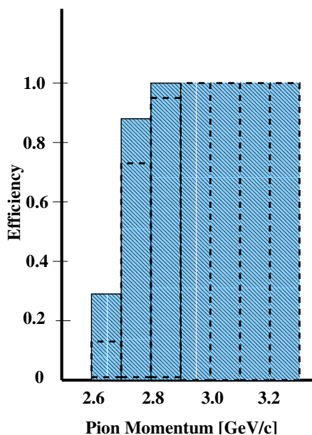
Figure 4.80: Predicted pion detection efficiency as a function of average pion momentum. The solid histogram is for a one-photoelectron detection threshold and the dashed line is for a two-photoelectron threshold.
