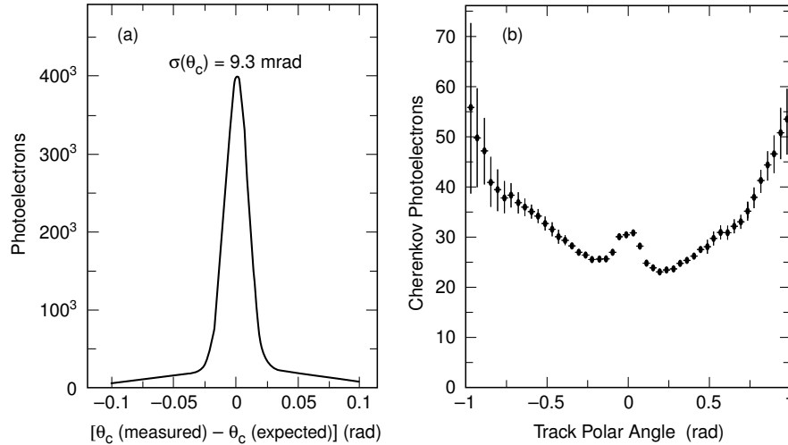
Figure 4.70: (a) The Cherenkov angle resolution for single photons associated with a particle track. (b) The number of Cherenkov photons per track versus the track polar angle with respect to normal incidence. The slightly lower efficiency in forward direction is due to the reflection in the mirror and the increased photon path-length in the bar.
