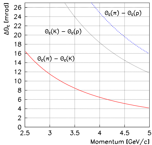
Figure 4.67: The difference in the Cherenkov angles between pions, kaons, and protons in synthetic quartz.
