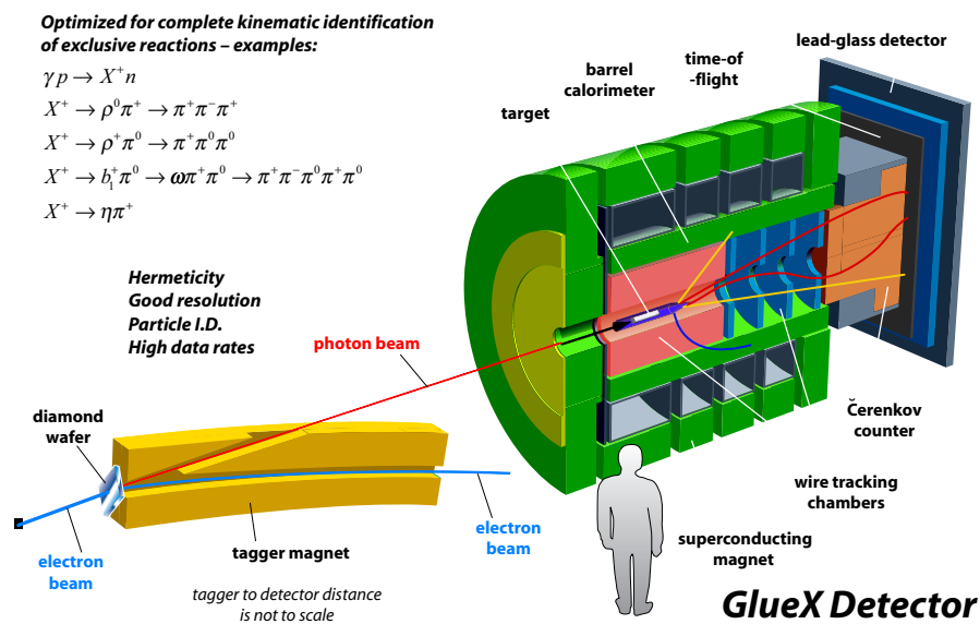
Figure 1.2: Schematic of the GLUEX/HALL D Detector.
