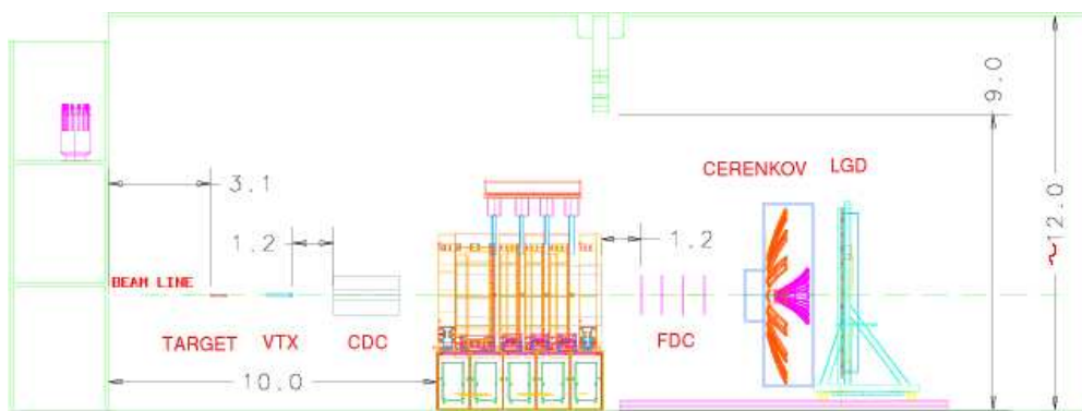
Figure 4.86: Exploded view of detector showing the detector subsystems in their extracted positions. The magnet does not move and detectors are inserted both from upstream and downstream into their nominal positions for normal operation.
