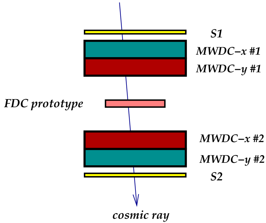
Figure 4.52: Schematic drawing of the cosmic-ray telescope used for FDC prototype resolution studies.
