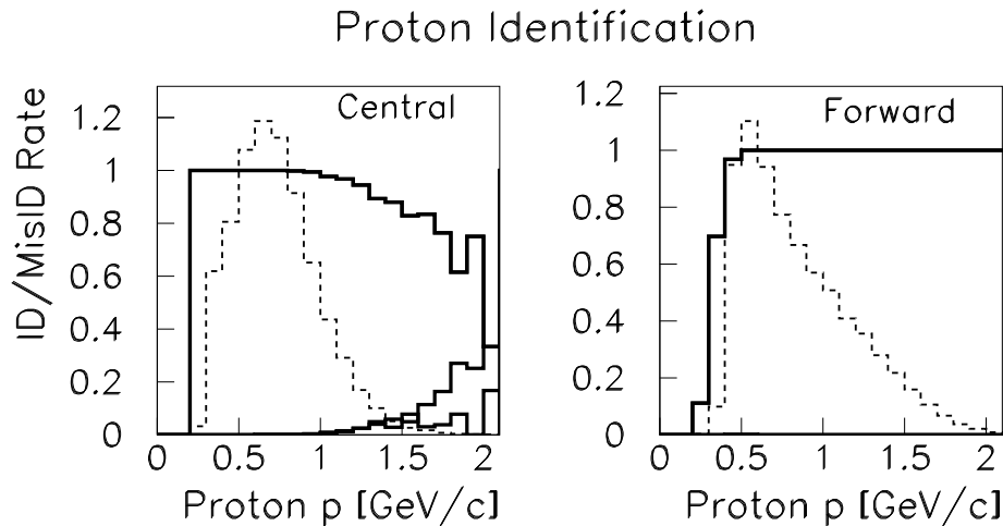
Figure 4.81: The acceptance of proton tracks in the reaction \gamma p \rightarrow K^* \bar{K}^* p . The left plot shows central tracks and the right plot shows forward tracks. The top curve is the correct identification rate; the bottom is the misID rate. The starting momentum spectra for proton tracks in the central or forward regions are shown in the background.
