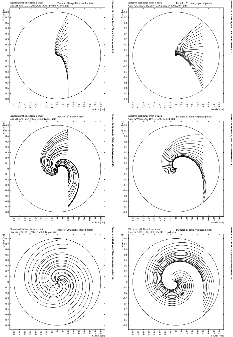
Figure 4.35: Garfield simulations of electrons drifting through a straw tube in the CDC. The curved shape of the tracks is due to the Lorentz angle induced by the 2.25 T magnetic field.
