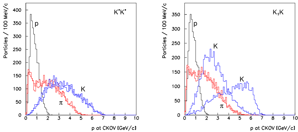
Figure 4.71: The particle momenta at the Cherenkov detector plane ( z = 450 cm) for the two reactions described in the text ( \pi :pions, K :kaons, p :protons).
