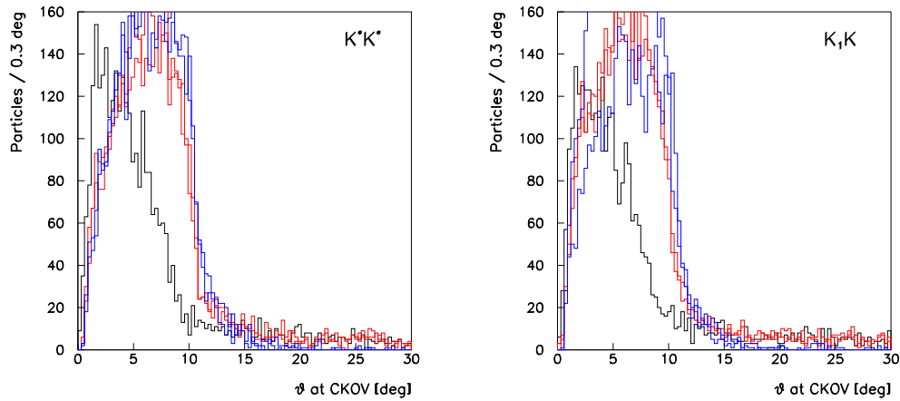
Figure 4.72: The polar angle with respect to the normal incidence at the Cherenkov detector plane ( z = 450 cm) for pions, kaons, and protons in the two reactions described in the text.
