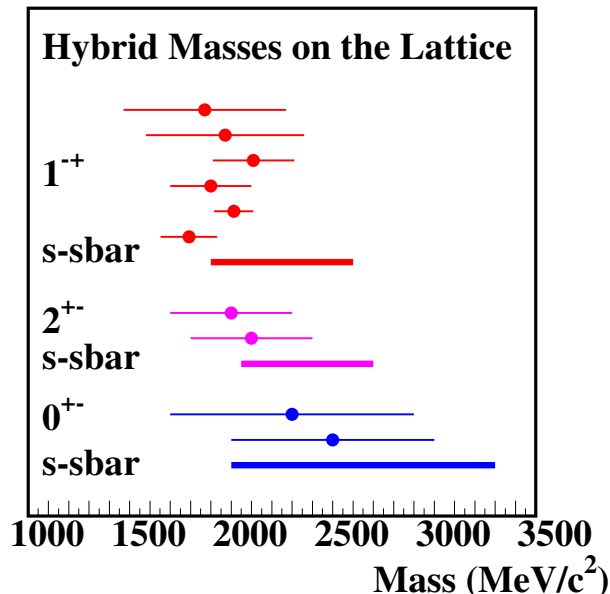
Figure 1: A graphical summary of the mass calculations for hybrids.
