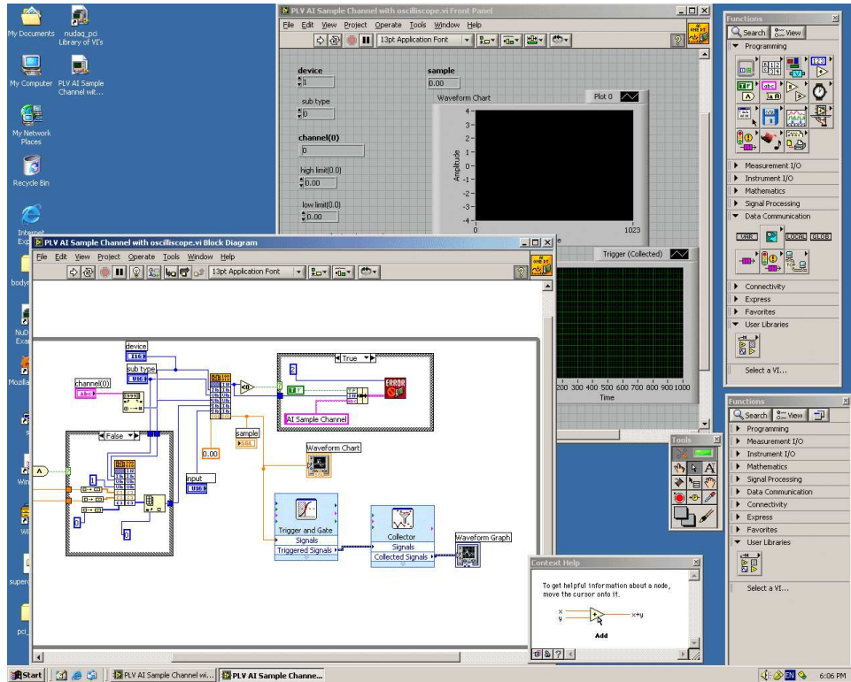
Figure 3: A screen shot of a Virtual Instrument in Labview. The window on the lower left provides a schematic of the data flow, including routines called, program flow control, triggering and the “back end” of the visual objects used to output the data. The window behind it shows the graphical run-time controls. The toolbars on the right are used to design the visual and back-end aspects of the virtual instruments.
