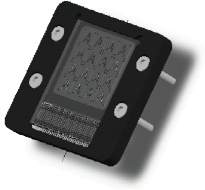
Fig. 4. A schematic drawing of possible SiPM package. The Phase-II packaging will not have a frame as thick as that shown in this figure, as that is not allowed by the close placement of the light collectors.
