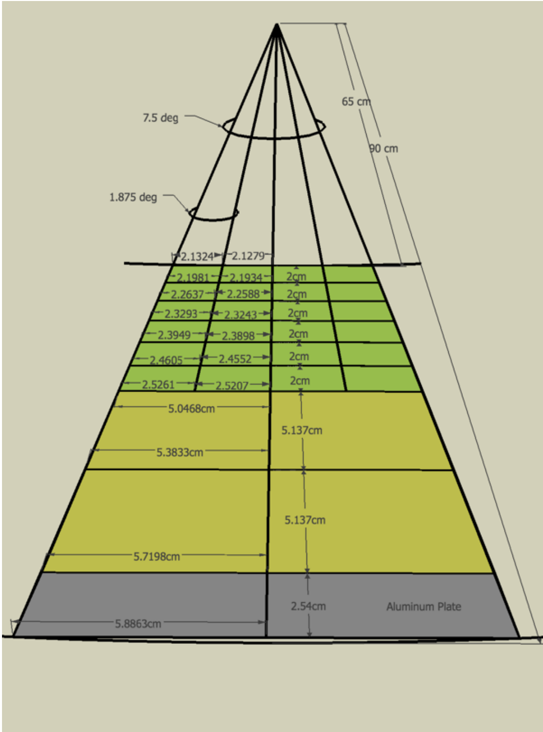
Fig. 3. Precise dimensions of the BCAL readout cells, for one side of one module. Note that the six inner layers each have a thickness of exactly 2 cm, whereas their trapezium sides vary, increasing from a bit over 2.1 cm to over 2.5 cm. The two outer layers have a thickness of 5.137 cm each. Only the left inner cells (with respect to the central \phi ray) are labeled for reasons of clarity. The right side is mirror-symmetric.
