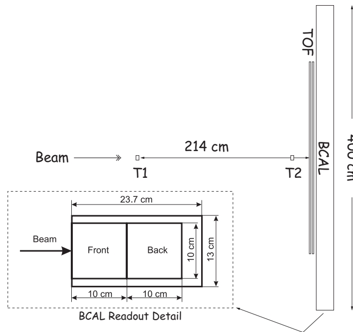
Figure 2.4: A schematic of the detector placement and readout for BCAL Module 1 for the beam tests at TRIUMF.
