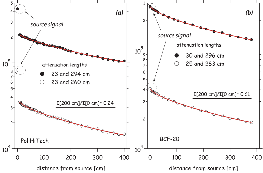
Figure 2.14: (a) Integrated spectrum as a function of distance from the source for the PolHiTech fiber before (filled circles) and after (open circles) convoluting the photon detection efficiency of the XP2020; (b) same for the BCF-20 fiber. The fits are to a double exponential with the short and long attenuation lengths quoted. The integrated signal at the source (at 0 cm) is indicated in the plots.
