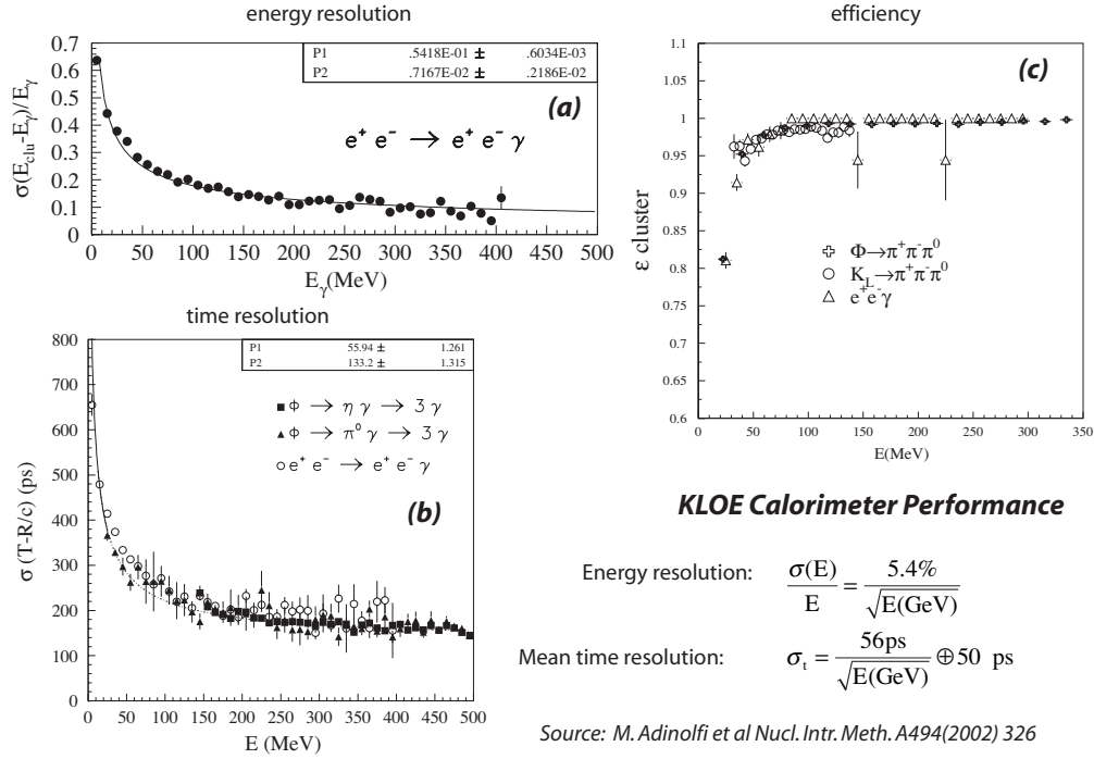
Figure A.2: Figures from reference [36]. (a) energy resolution as a function of energy; (b) time resolution as a function of energy; and (c) photon detection efficiency as a function of energy.
