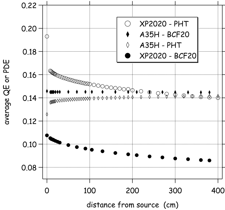
Figure 2.15: The average QE of the XP2020 and the average PDE of the A35H as a function of distance from source for PolHiTech (PHT) and BCF20 scintillating fibers. Details are given in the text.
