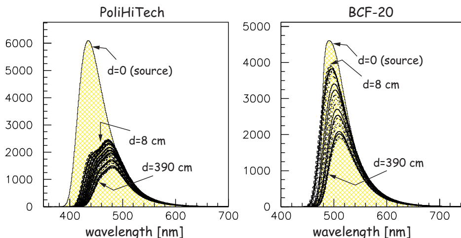
Figure 2.13: The Moyal representations of the source and measured spectra for the PolHiTech and BCF-20 fibers. The source spectra (filled yellow) were normalized to match the 8 cm measured spectra at 550 nm for the BCF-20 fiber and at 520 nm for the PolHiTech fiber.
