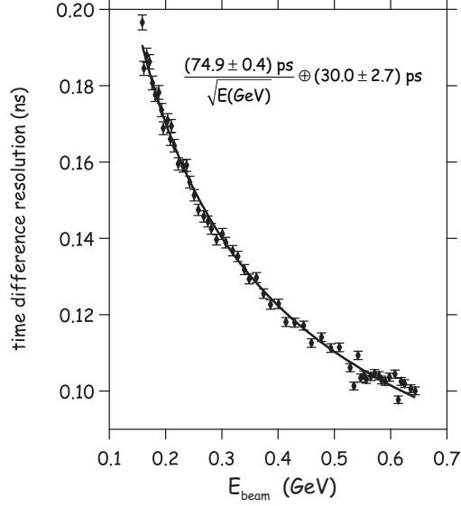
Figure 2.10: The time difference resolution as a function of beam energy. The time difference resolution is obtained by fitting the distribution in \Delta t = t_S - t_N , the North-South time difference, to a Gaussian for bins of beam energy.
