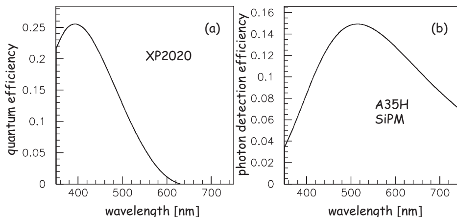
Figure 2.12: The photon detection efficiency over the range of relevant wavelengths for the (a) Amperex XP2020 and the (b) SensL silicon photomultiplier A35H at +2V above breakdown voltage.
