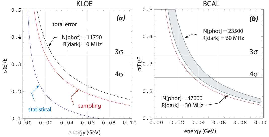
Figure 2.16: The relative error in energy measurement, \sigma(E)/E as a function of energy for (a) KLOE parameters and (b) BCAL parameters. In (a) the contributions from the statistical and sampling terms are shown in blue and red. The total error includes these two terms added in quadrature along with a constant floor term of 1%. In (b) two different assumptions about photon yield and dark rate are shown. For both we assume f_{PDE} = 0.12 . More details are given in the text.
