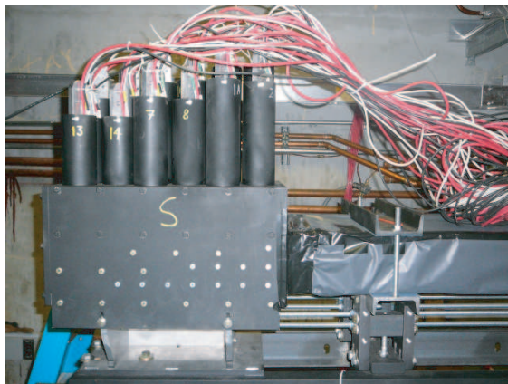
Figure 2.8: The black box encloses the 18 light guides and PMTs with cables attached for the South end of the BCAL module and is similar to the North end. The BCAL Pb/Sci-Fi matrix is wrapped in Teflon on the right and pressed against the light guides coupled with a silicone cookie.
