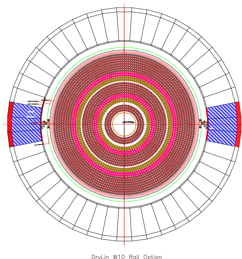
Figure 18: The CDC sitting on support rails in the final GlueX detector.
