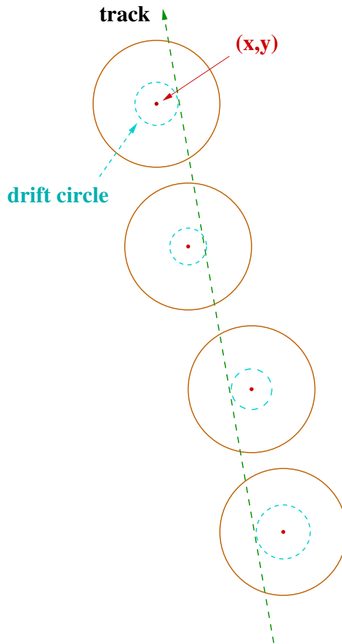
Figure 25: A track going through four straw tubes in the CDC. The straw tubes are shown as the large circles and the location of the wire is indicated as the dot at the center of the circles. The track passes through the wires and the first ionization in each tube comes from the point where the track intersects the dashed circle inside the straw tube. For each hit, we then have the (x, y) coordinate of the wire and the radius of the dashed circle.
