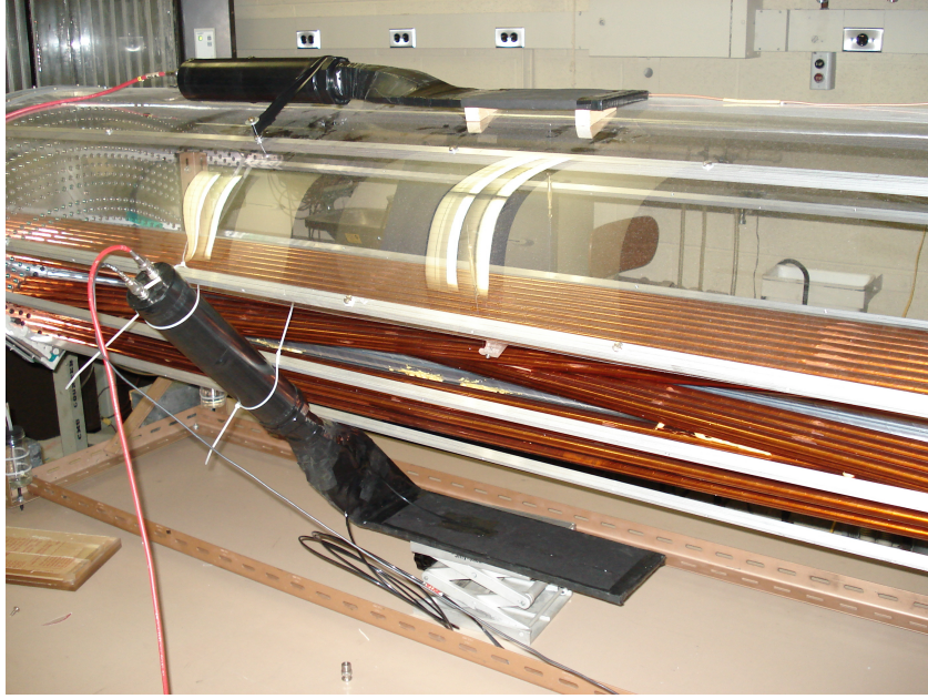
Figure 20: A photograph of the 2 m long CDC prototype at Carnegie Mellon. The copper-colored tubes are kapton and the silver-colored ones are mylar. Also shown are a pair of scintillators used in a specialized cosmic trigger.
