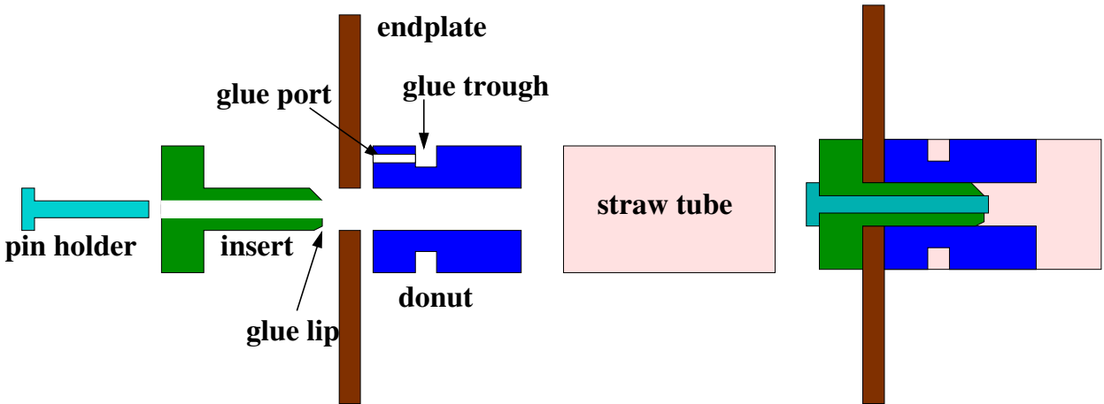
Figure 6: The CMU designed feed throughs which provide a solid glue joint between the straw-tube and the end plate. The left-hand figure shows an expanded view, while the right-hand shows the feed throughs in the chamber end plates.
