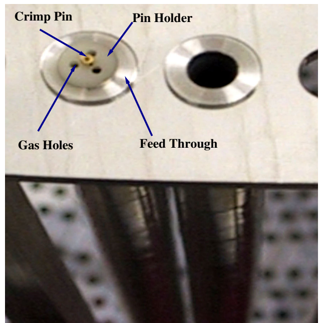
Figure 15: (left) Shows a donut being glued into a straw tube. (right) Shows the feed throughs holding a straw tube in place at the end of the chamber. Note the crimp pin in the center of the pin holder and the three holes to allow gas to flow into the straw tube.
