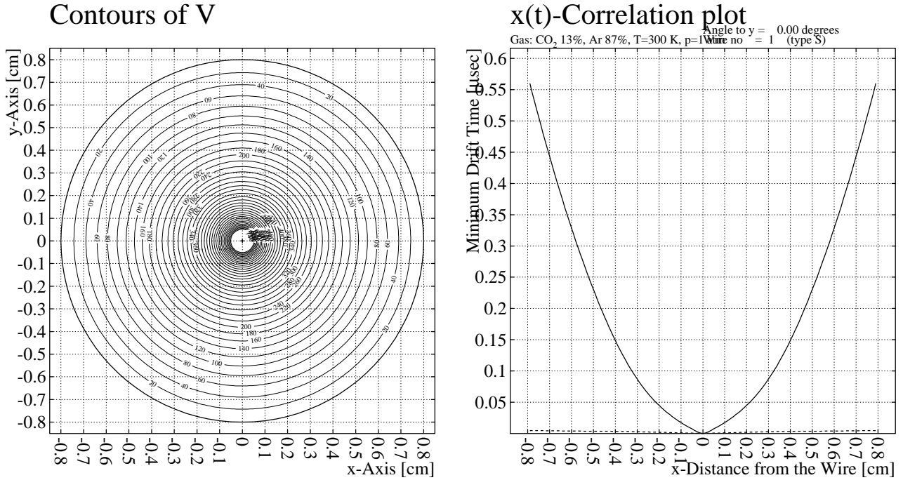
Figure 7: The left-hand plot shows a GARFIELD [1] calculation of the electric field in the straw tube. The right-hand figure shows a typical time-to-distance plot calculated for the straw-tube geometry in the 2.24 T magnetic field.
