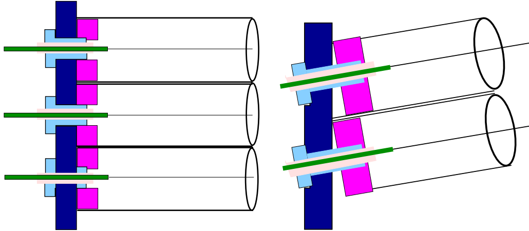
Figure 5: A schematic drawings of the feed throughs for both the normal ( left ) and stereo ( right ) wires in the CDC.
