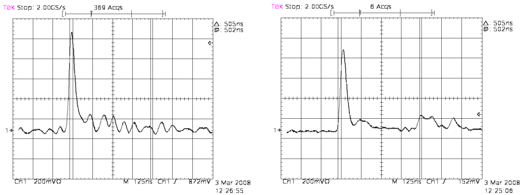
Figure 21: (left) A signal pulse as seen on a straw before work on grounding and noise reduction. (right) A signal pulse after improvements. Both plots are on a 200\text{ mV} per division scale. Note the noise at nearly 100\text{ mV} peak-to-peak before reduction. After reduction, the noise is essentially invisible on the trace. Note that the left-hand trace shows a second pulse about 400\text{ ns} after the primary, the noise level is only visible on the few \text{mV} scale.
