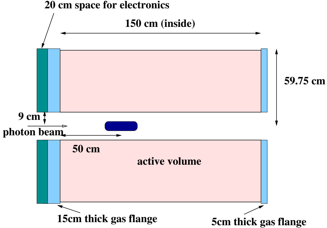
Figure 2: A side view of the CDC. The active region is 150 cm long with a 0.6 cm thick downstream end plate and a 0.9 cm thick up-stream end plate. At the downstream end is a 5 cm thick gas plenum which collects the gas from the tubes. At the upstream end a 15 cm thick plenum for distributing gas and then an additional 20 cm of space for electronics. All cables will be taken off the up-stream end of the chamber. The inner and outer radius of the end plates are 9 cm and 59.75 cm respectively.
