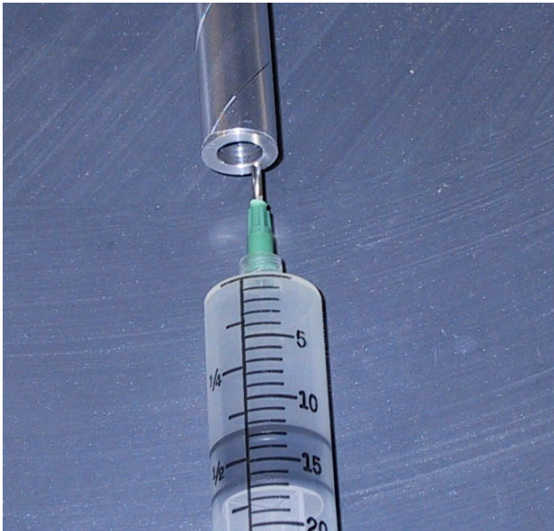
Figure 15: (left) Shows a donut being glued into a straw tube. (right) Shows the feed throughs holding a straw tube in place at the end of the chamber. Note the crimp pin in the center of the pin holder and the three holes to allow gas to flow into the straw tube.
