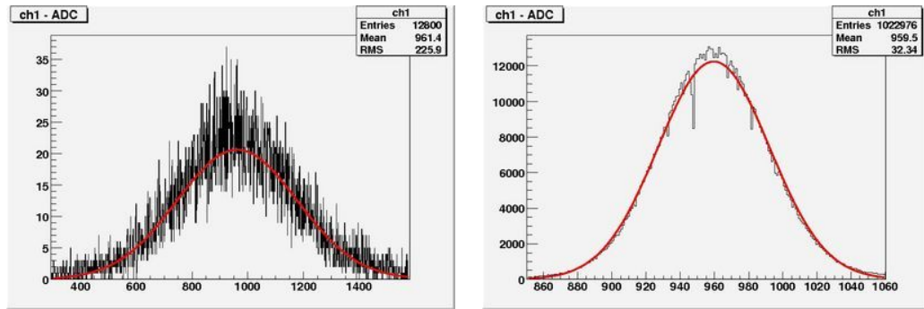
Figure 23: (left) The pedestal on a straw before work on grounding and noise reduction. (right) The pedestal on the same channel after improvements. Note that the final pedestal is significantly narrower than what it was originally.
