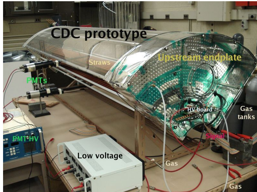
Figure 19: A photograph of the 2\text{ m} long CDC prototype at Carnegie Mellon. The copper-colored tubes are kapton and the silver-colored ones are mylar. Also shown are a pair of small scintillators used in a specialized cosmic trigger.
