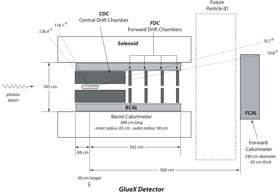
Figure 1: A cut-away view of the GlueX detector. The Central Drift Chamber (CDC) is shown as the cylindrical chamber around the target. The Forward Drift Chamber packages are shown downstream of the CDC.
