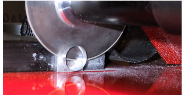
Figure 14: The high-speed saw used to cut the CDC straw tubes to the appropriate length. The black knob on the left-side of the saw tightens a clamp that holds the tubes in place for cutting. The right-hand picture shows a mylar straw being cut by the saw.
