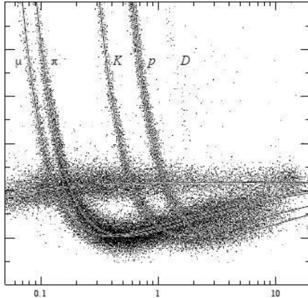
Figure 26: PEP4/9-TPC energy-deposit measurements (185 samples @8.5 atm Ar-CH4 80%20% ) in multihadron events. Plot taken from the 2006 edition of the Particle Data Book.
