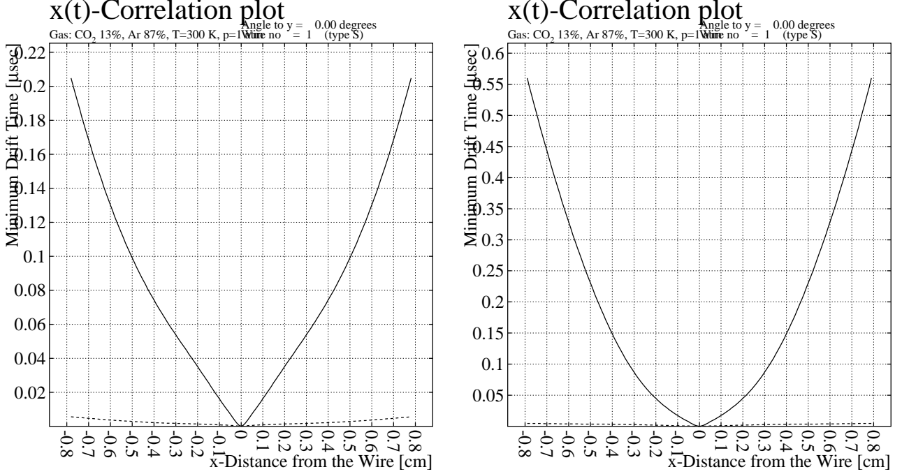
Figure 9: Calculated time versus distance in 87% Argon, 13% Carbon Dioxide mixture. left: No magnetic field, right: full magnetic field. Both plots are for 1800 V on the anode wire.
