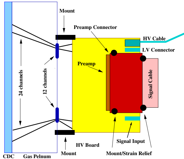
Figure 15: A conceptual drawing of the high-voltage board and preamp mounted on the downstream gas plenum and connected to the CDC via a pair of custom feed throughs.
