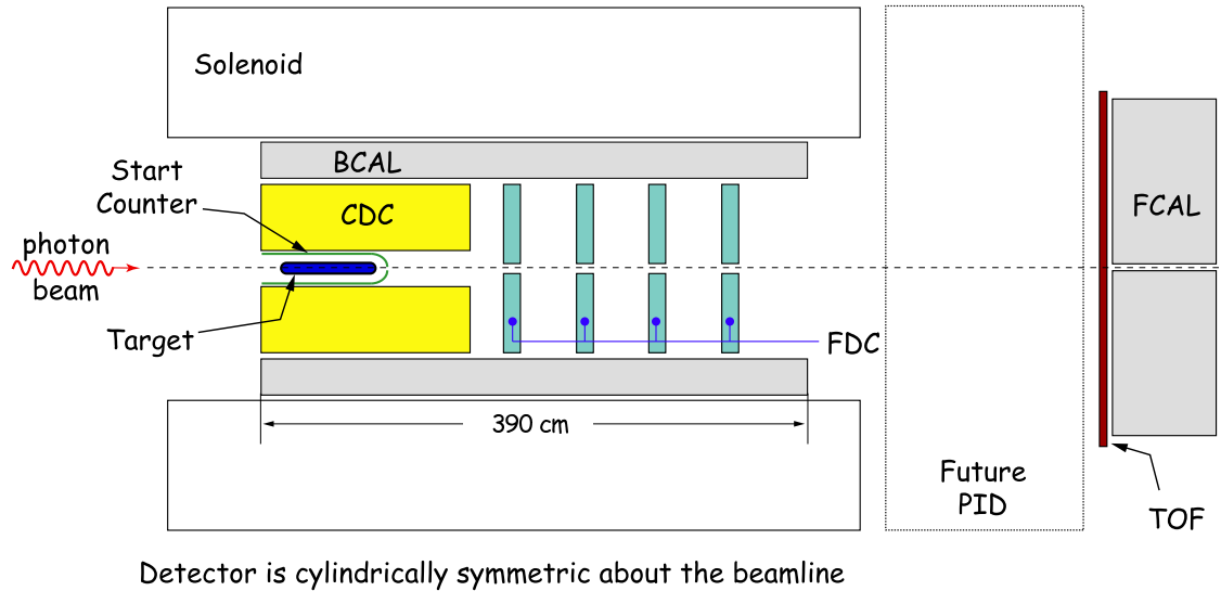
Figure 1: Schematic of the GLUEX detector. A description is provided in the text.
