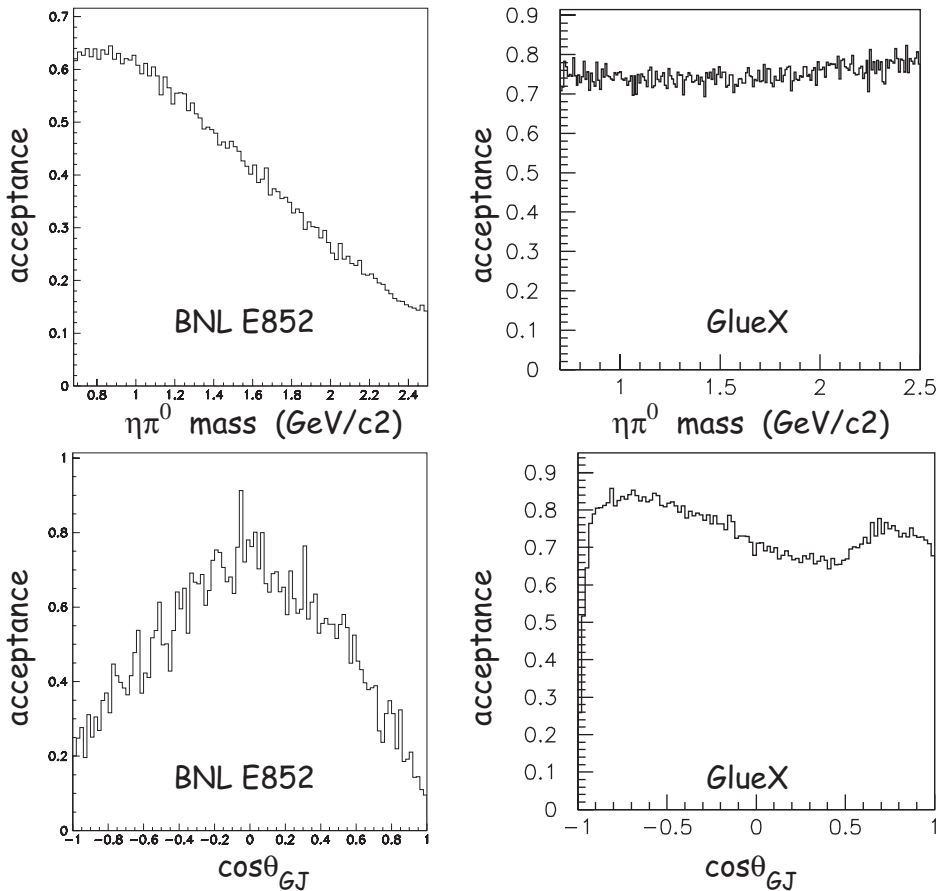
Figure 20: A comparison of the expected acceptance of the GLUEX detector for the reaction \gamma p \rightarrow p\eta\pi^0 with the acceptance of the E852 experiment. The upper two plots show the acceptance as a function of the mass of the \eta\pi system, while the lower two plots show the acceptance as a function of the Gottfried-Jackson angle.
