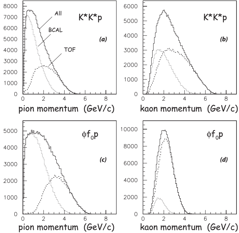
Figure 32: Momentum spectra shown separately for \pi^\pm and K^\pm for the final states K^*(890)\bar{K}^*(890)p and \phi f_0(980)p . The light dashed histograms are for particle hitting the BCAL and the darker dashed for the forward time-of-flight, while the solid histograms are the sum (figure taken from reference [46]).
