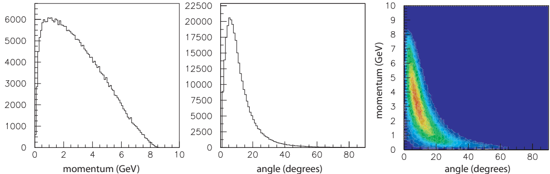
Figure 26: The momentum and angle spectra of charged pions and their correlation from the reaction \gamma p \rightarrow \pi^+ \pi^+ \pi^- n for 8.5 to 9.0 GeV photons (figure taken from reference [46]).
