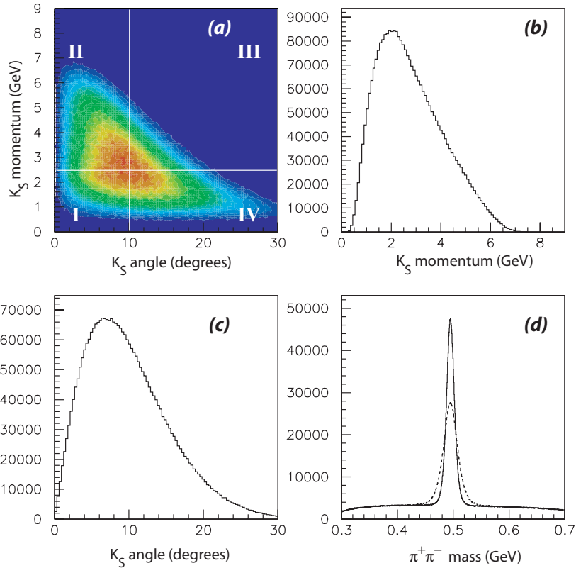
Figure 5: Kinematics of the K_S^0 for the reaction \gamma p \rightarrow K_S^0 \pi^+ K_S^0 \pi^- p . Please see text for details (figure taken from reference [24]).
