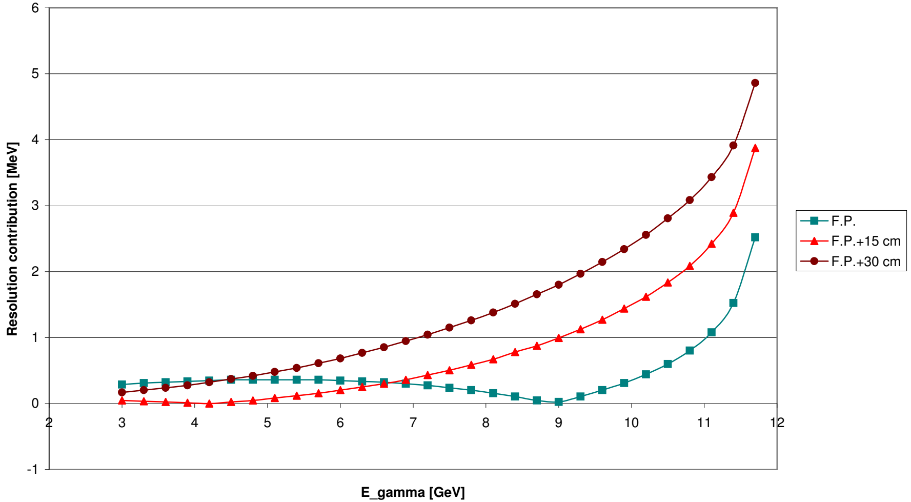
Effect of fixed array displacement on energy resolution (counter energy width is typically 15-25 MeV)
