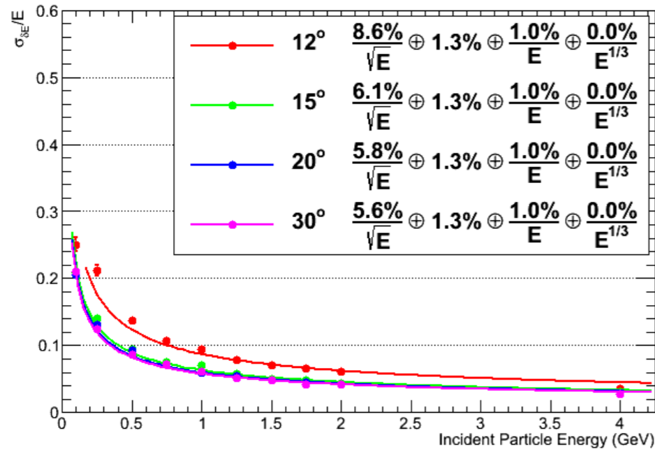
BCAL Energy resolution from M.C. September 20, 2012 DL svn revision 9396
