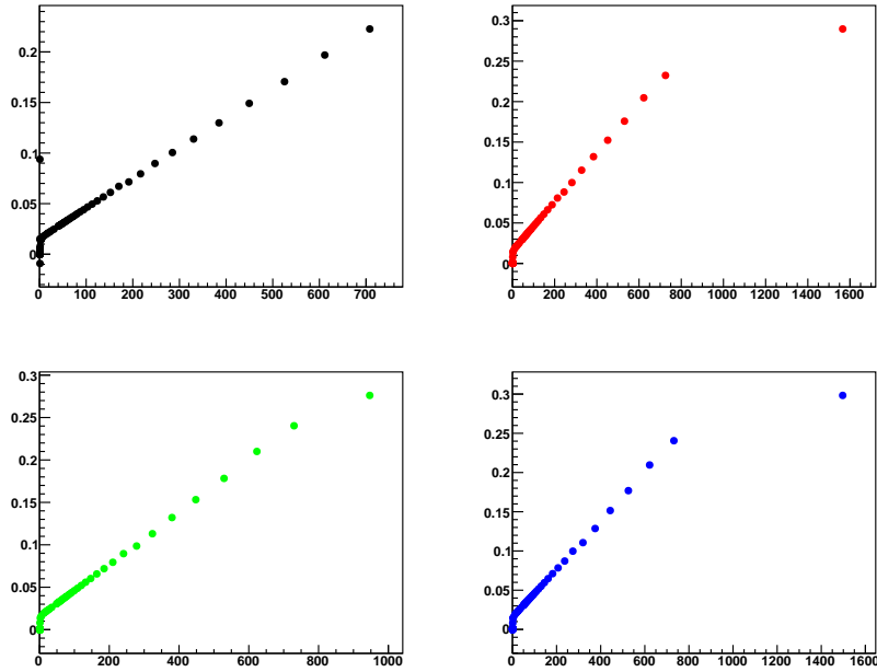
Figure 17: APD AA4654. \left(\frac{1}{G} \frac{dG}{dV}\right) [V -1 ] vs G at four different temperatures.
