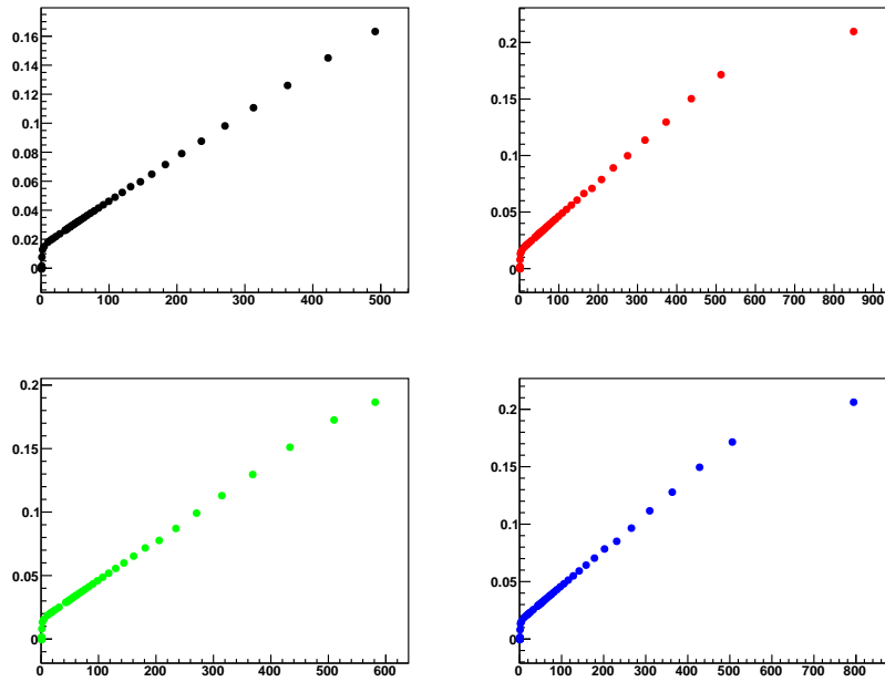
Figure 27: APD AA4655. \left(\frac{1}{G} \frac{dG}{dV}\right) [\text{V}^{-1}] vs G at four different temperatures.
