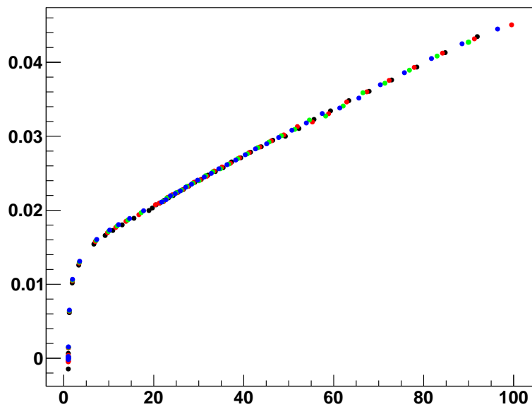
Figure 8: APD 0605004458. \left(\frac{1}{G} \frac{dG}{dV}\right) [\text{V}^{-1}] vs G with four temperatures superimposed.
