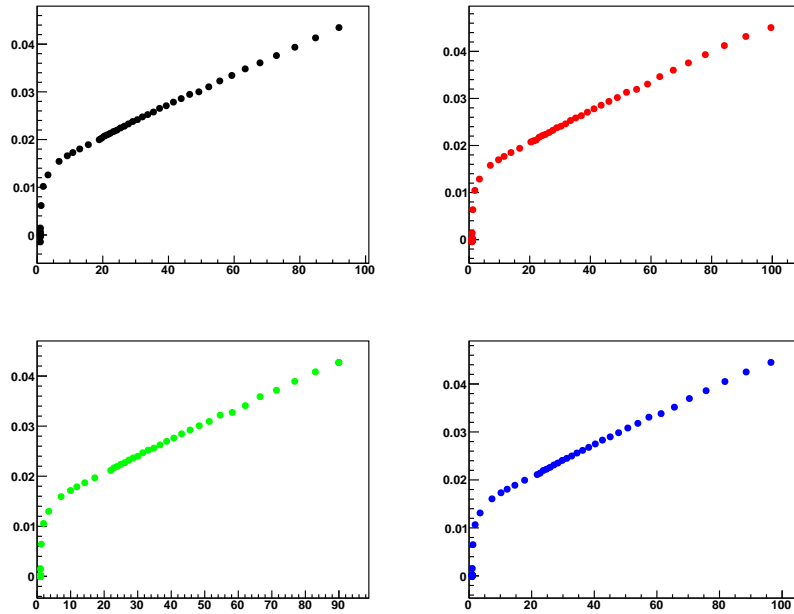
Figure 7: APD 0605004458. \left(\frac{1}{G} \frac{dG}{dV}\right) [\text{V}^{-1}] vs G at four different temperatures.
