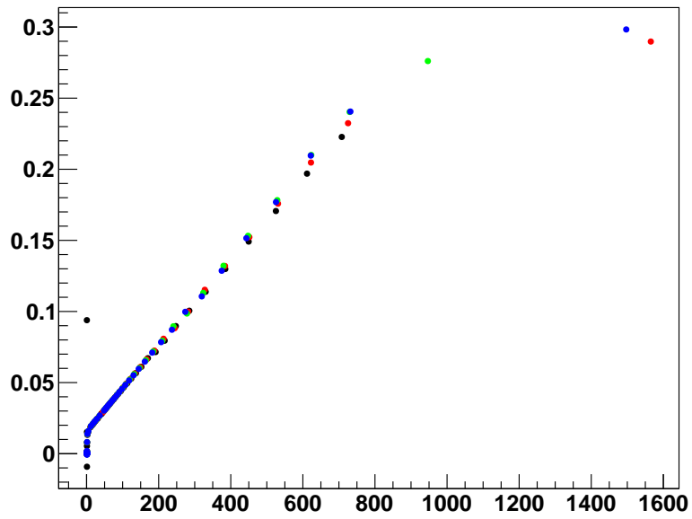
Figure 18: APD AA4654. \left(\frac{1}{G} \frac{dG}{dV}\right) [V -1 ] vs G with four temperatures superimposed.
