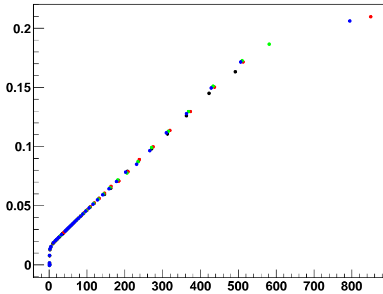
Figure 28: APD AA4655. \left(\frac{1}{G} \frac{dG}{dV}\right) [\text{V}^{-1}] vs G with four temperatures superimposed.
