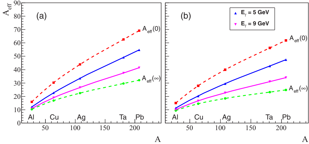
FIG. 1. Dependence of the nuclear transparency A_{\text{eff}} on the mass number for (a) \sigma_L = 13 mb and (b) \sigma_L = 26 mb. A_{\text{eff}} is shown for different photon energies: A_{\text{eff}}(\infty) and A_{\text{eff}}(0) correspond to infinite energy and energy-independent transparency, respectively.
