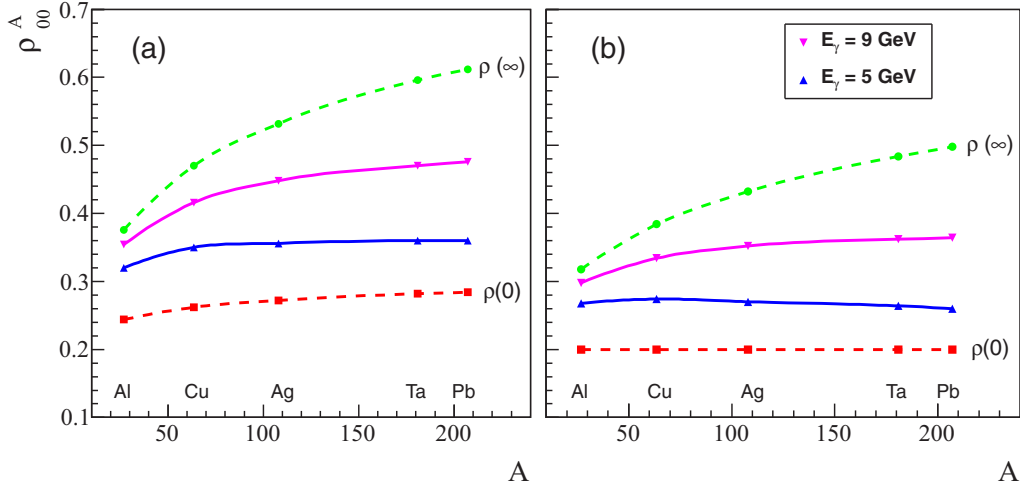
FIG. 2. A dependence of the spin density matrix element \rho_{00}^A for (a) \sigma_L = 13 mb and (b) \sigma_L = 26 mb. \rho_{00}^A is shown for different photon energies: \rho(\infty) and \rho(0) correspond to infinite energy and energy-independent \rho_{00}^A , respectively.
