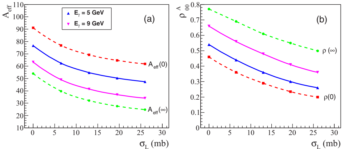
FIG. 3. (a) The nuclear transparency A_{\text{eff}} and (b) the spin density matrix element \rho_{00}^A as a function of \sigma_L for lead nucleus. The transverse \omega -nucleon cross section \sigma_T and the spin density matrix element \rho_{00} are taken to be 26 mb and 0.2, respectively.
