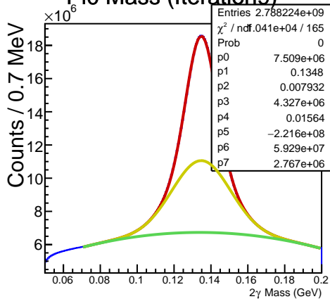
Pi0 Mass (Iteration9)
