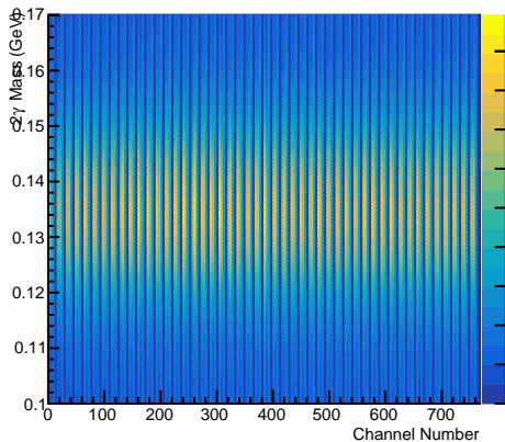
Pi0 Mass vs. Channel Number (Iteration17)
