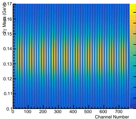
Pi0 Mass vs. Channel Number (Iteration23)
