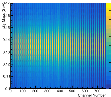
Pi0 Mass vs. Channel Number (Iteration19)
