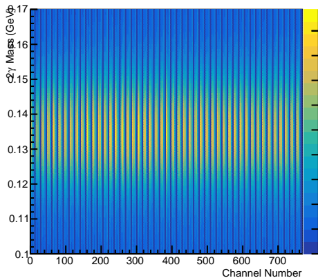
Pi0 Mass vs. Channel Number (Iteration16)
