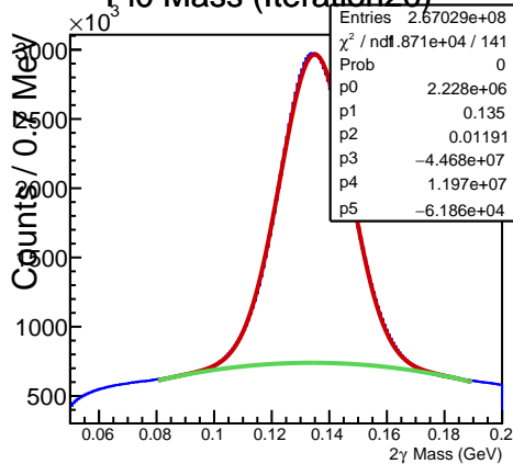
Pi0 Mass (Iteration20)
