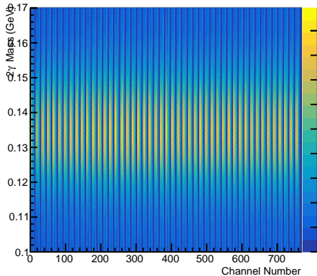
Pi0 Mass vs. Channel Number (Iteration18)
