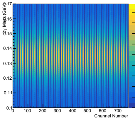
Pi0 Mass vs. Channel Number (Iteration24)
