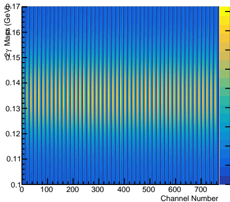
Pi0 Mass vs. Channel Number (Iteration14)
