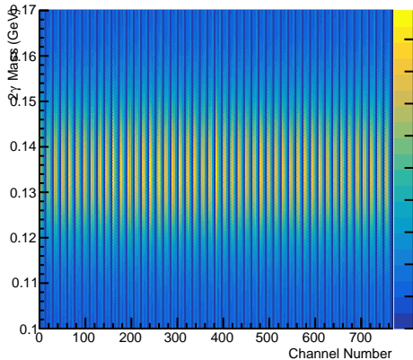
Pi0 Mass vs. Channel Number (Iteration21)
