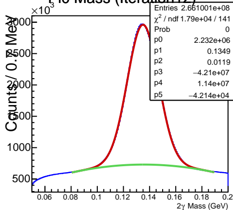
Pi0 Mass (Iteration12)
