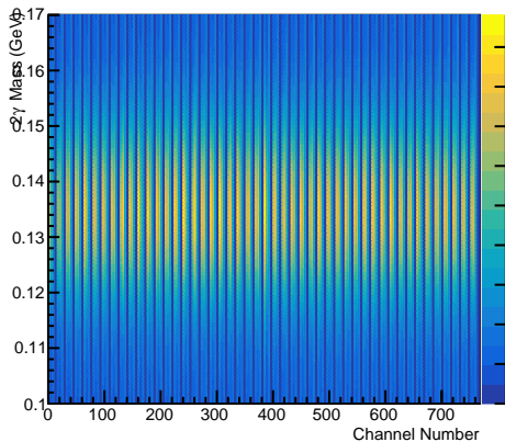
Pi0 Mass vs. Channel Number (Iteration22)
