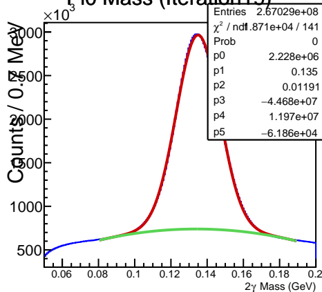
Pi0 Mass (Iteration19)
