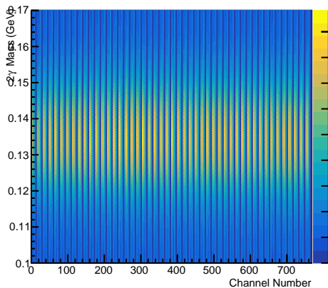
Pi0 Mass vs. Channel Number (Iteration15)
