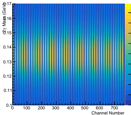
Pi0 Mass vs. Channel Number (Iteration20)
