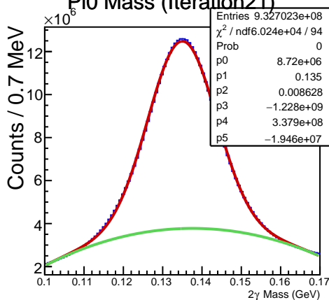
Pi0 Mass (Iteration21)
