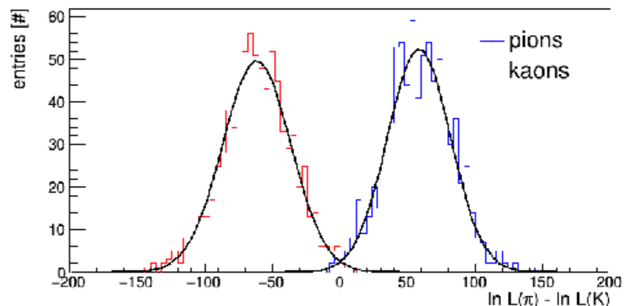
\pi/K separation power
