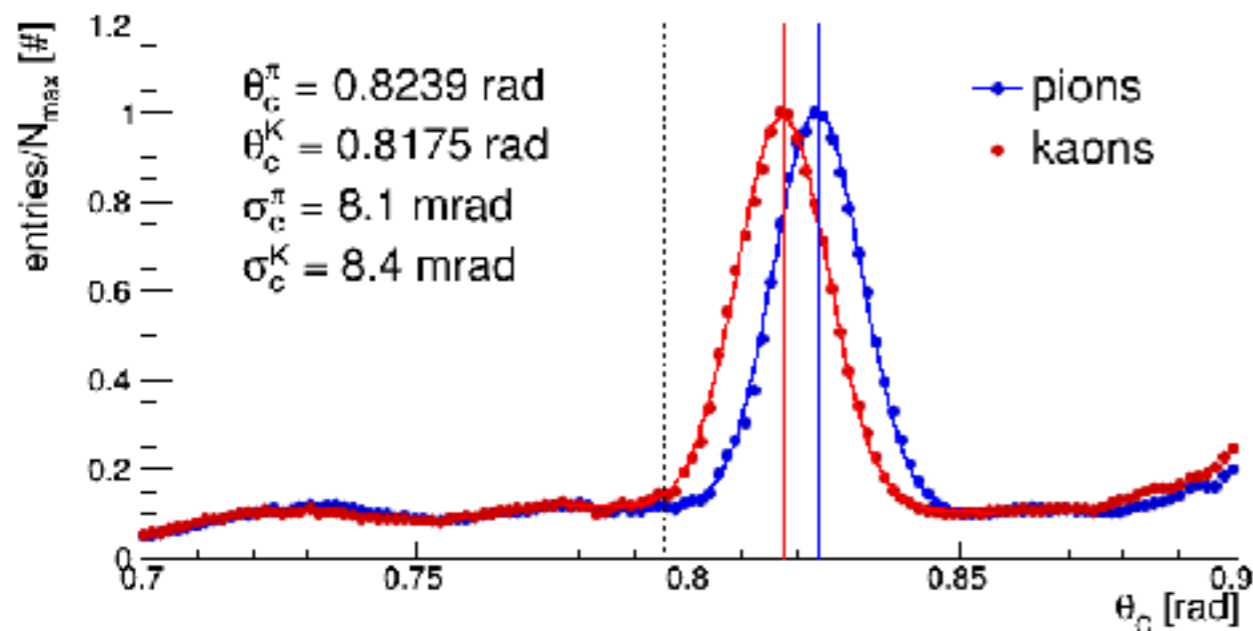
Single photon \theta_c resolution
