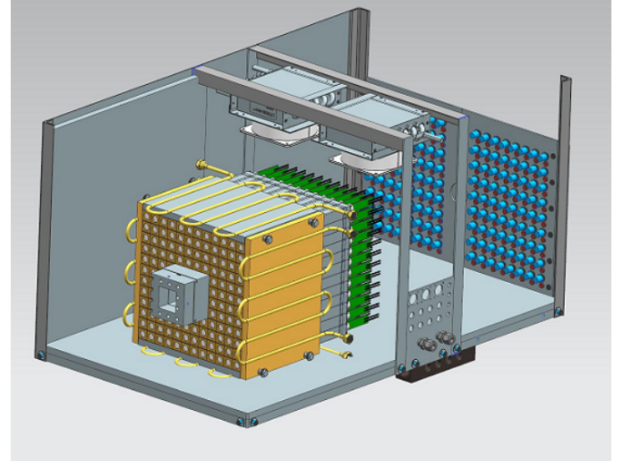
Figure 2: Schematic layout of the Compton calorimeter.
