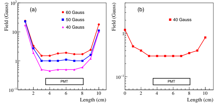
Figure 14: Magnetic field distribution inside the shield housing as a function of the distance from the housing face. Plot (a) corresponds to the longitudinal field and plot (b) corresponds to the transverse field. Markers correspond to different fields produced by Helmholtz coils.
