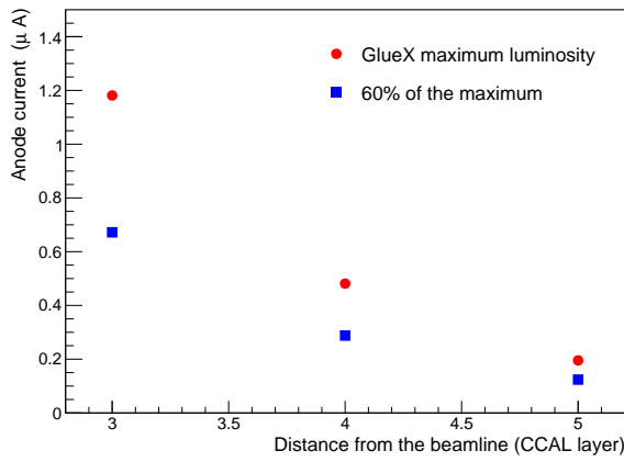
Figure 16: PMT anode current of CCAL modules for different layers.
