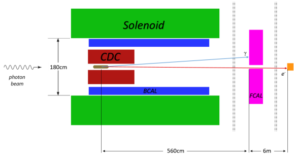
Figure 3: Schematic layout of the GlueX detector.
