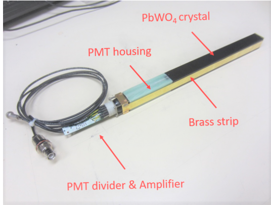
Figure 1: Calorimeter module.
