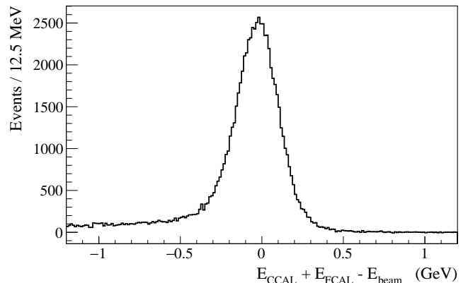
Figure 14: Elasticity distribution of reconstructed Compton candidates. The elasticity is defined as the energy of two clusters in the calorimeters minus the beam energy.
