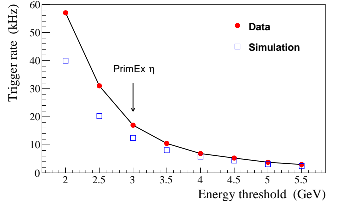
Figure 11: Trigger rate as a function of the total energy deposited in the FCAL and CCAL. Circles represent data and boxes represent the rate of electromagnetic interactions predicted by Monte Carlo simulation. The arrow indicates the energy threshold used in PrimEx- \eta production runs.
