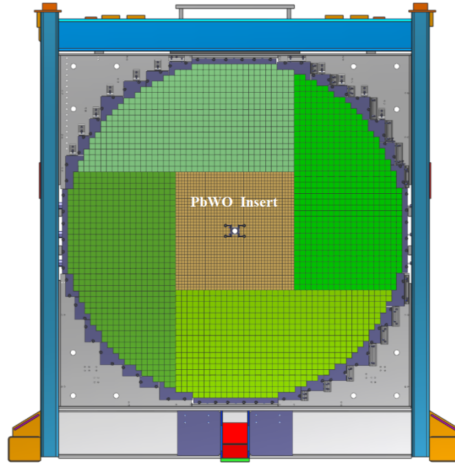
Figure 1: The forward calorimeter of the GlueX detector. Brown and green colors denote FCAL regions instrumented with \text{PbWO}_4 crystals and lead glass blocks. The photon beam passes through the hole in the middle of the calorimeter. The plot is taken from Ref. [17].
