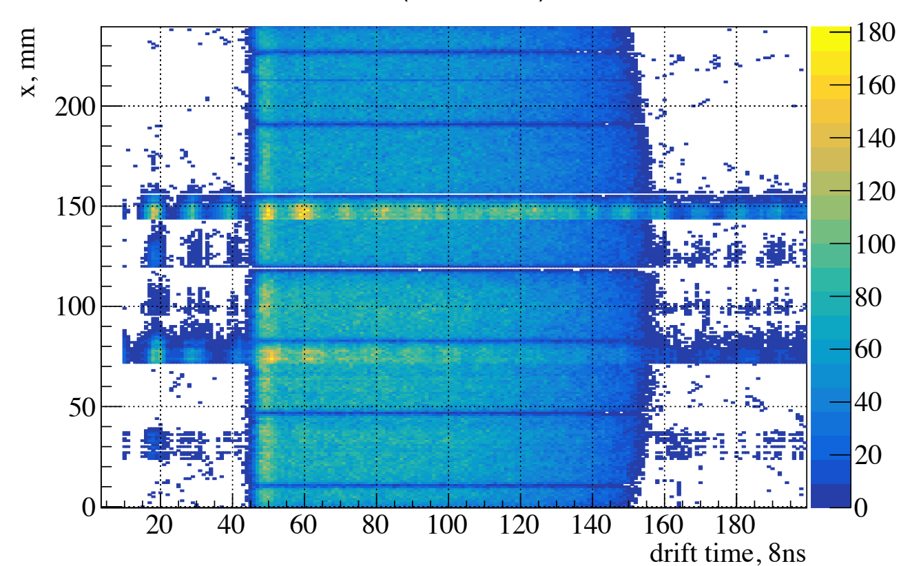
Ch.2 Width (transverse) vs Time
