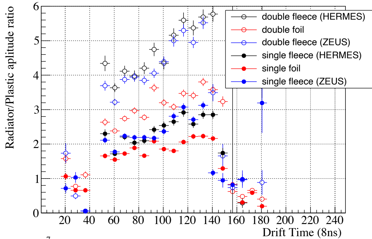
Radiator/plastic amplitude ratio
