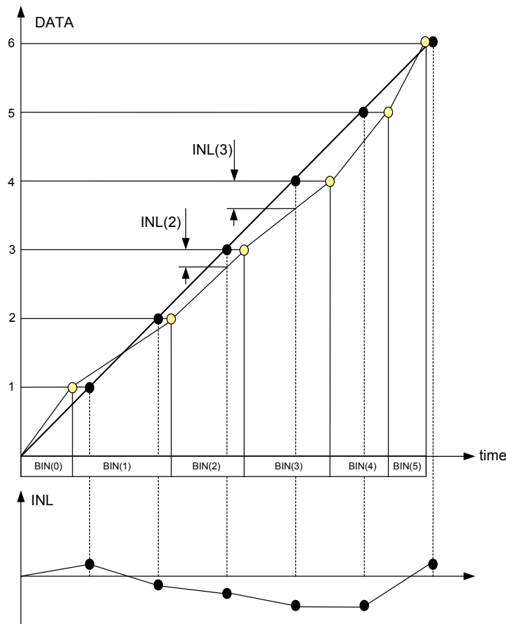
Fig. 2.9 INL I/O Characteristic
