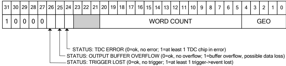
Fig. 6.7: Output Buffer: the Trailer
