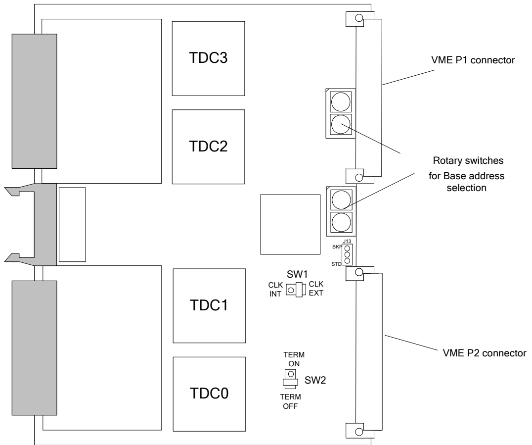
Fig. 3.3: Component Location (V1290 A 4 )
