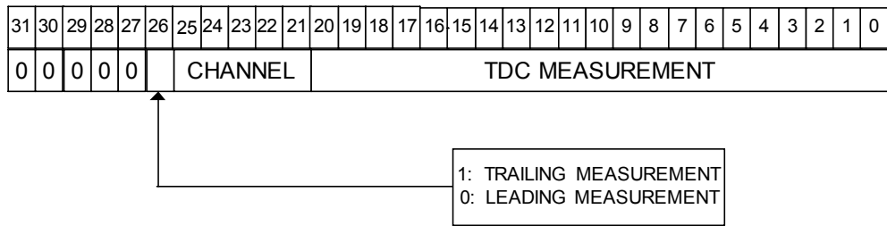
Fig. 6.2: Output Buffer: the TDC Header
