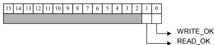
Fig. 6.27: Micro Handshake register
