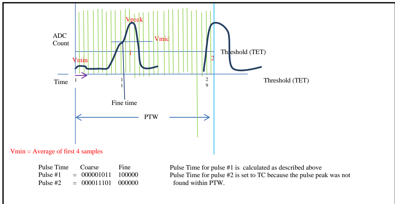
Figure 3: TDC
