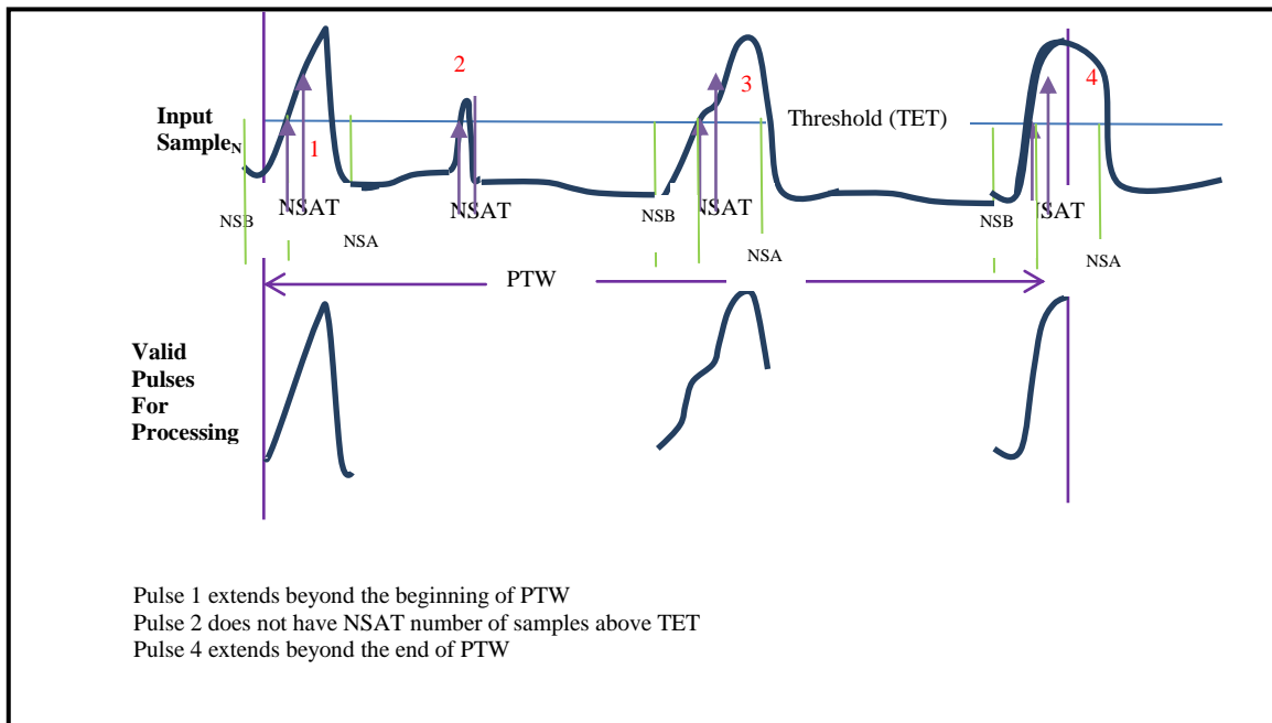
Figure 2 : Pulse Definition
