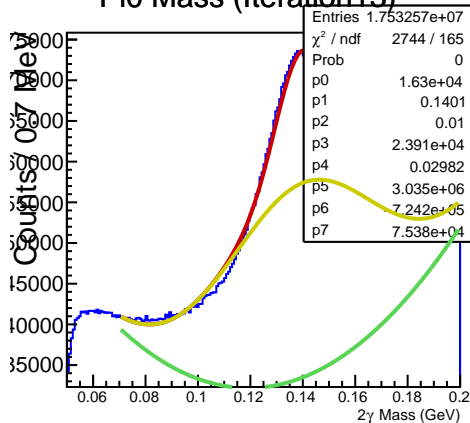
Pi0 Mass (Iteration 13)
