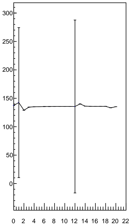
2 \gamma fit mean vs. Iteration
