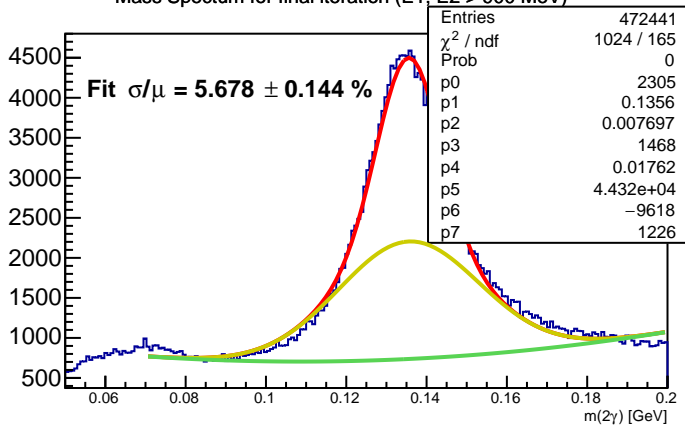
Mass Spectrum for final iteration (E1, E2 > 900 MeV)
