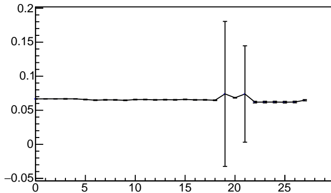
\sigma/\mu vs. Iteration (E1, E2 > 500 MeV)
