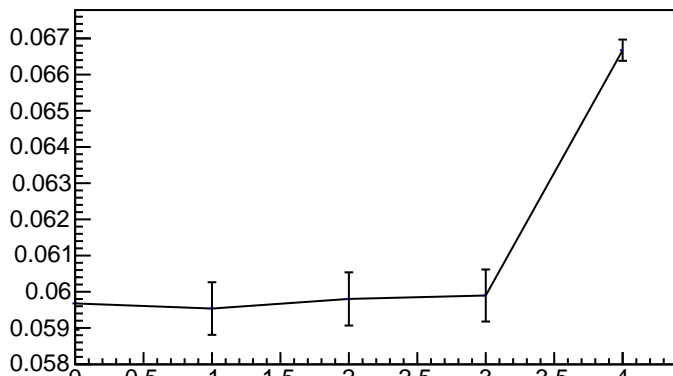
\sigma/\mu vs. Iteration (E1, E2 > 700 MeV)
