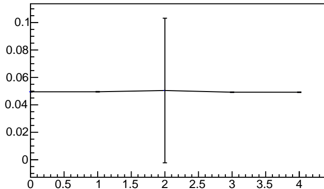
\sigma/\mu vs. Iteration (E1, E2 > 1100 MeV)
