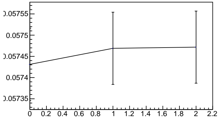
\sigma/\mu vs. Iteration (E1, E2 > 500 MeV)
