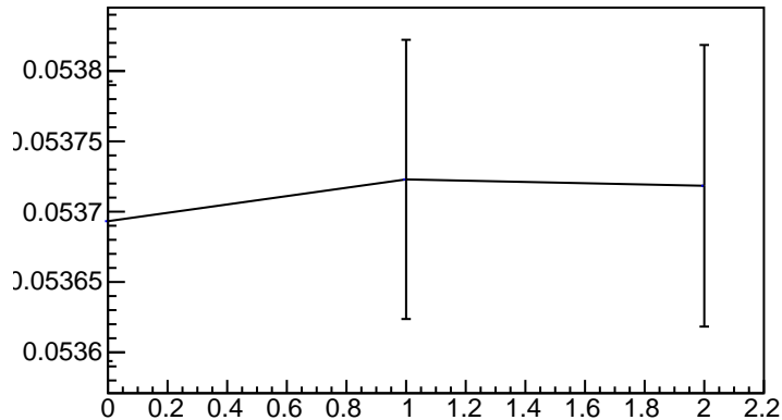
\sigma/\mu vs. Iteration (E1, E2 > 700 MeV)
