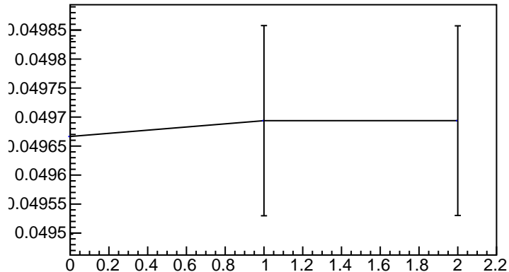
\sigma/\mu vs. Iteration (E1, E2 > 1100 MeV)
