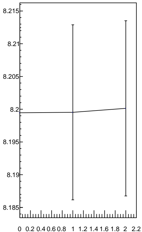
2 \gamma fit sigma vs. Iteration
