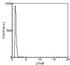
● \chi^2 distribution
