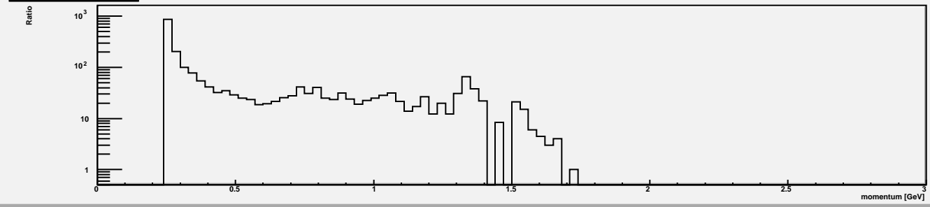
pi_yield/k_yield z=122
