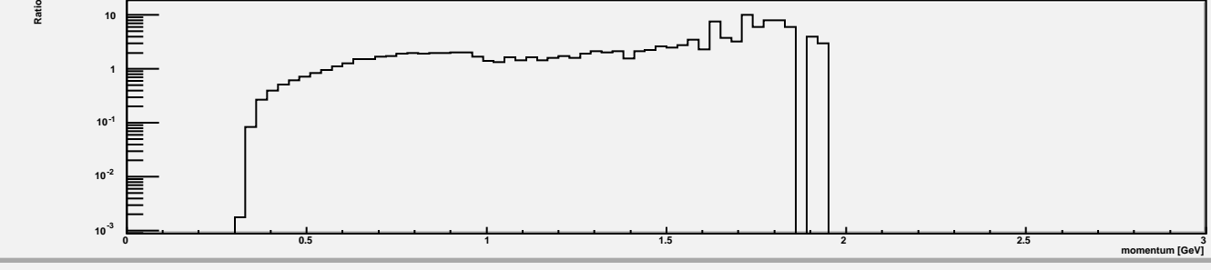
P_yield/k_yield z=122
