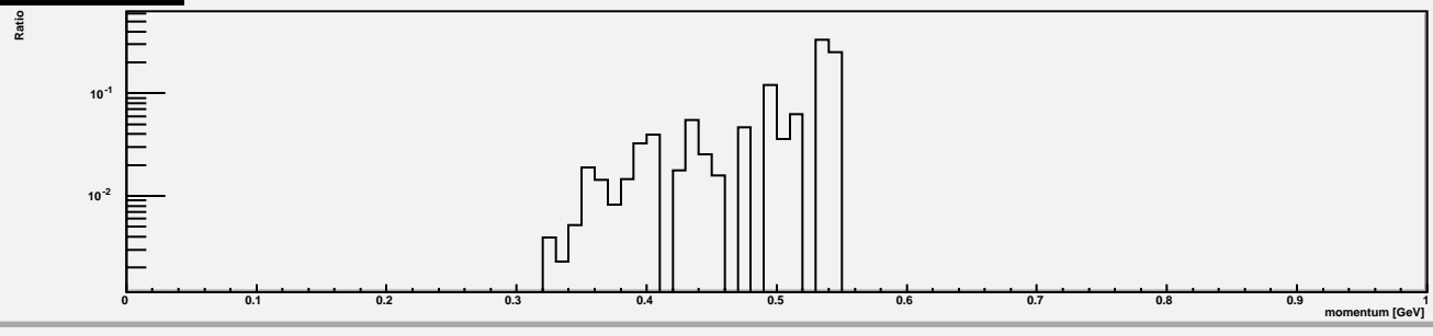
P_yield/k_yield z=32
