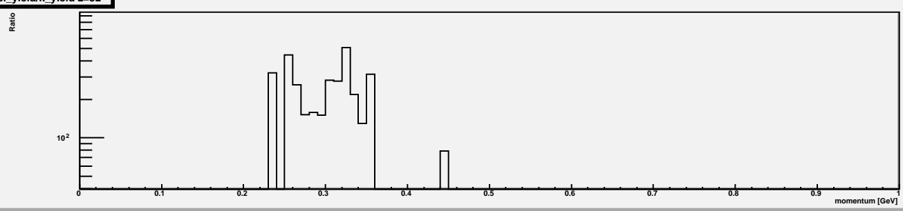
pi_yield/k_yield z=32
