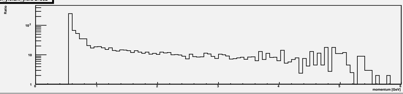
pi_yield/k_yield z=332
