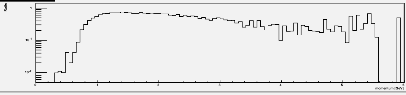
P_yield/k_yield z=332
