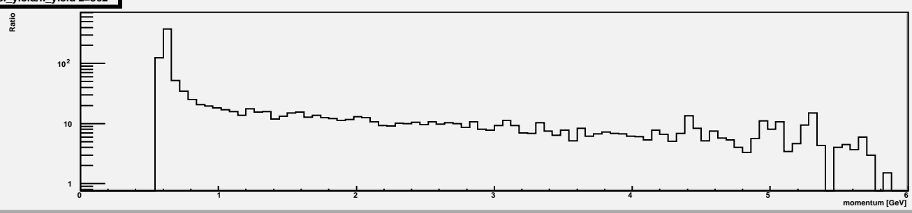
pi_yield/k_yield z=362
