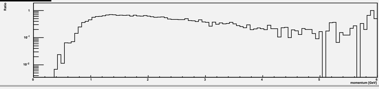
P_yield/k_yield z=362
