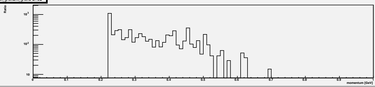
pi_yield/k_yield z=62
