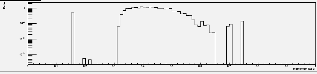
P_yield/k_yield z=62
