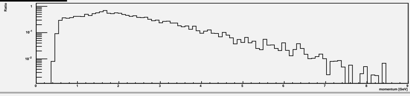
P_yield/k_yield alpha=1.75
