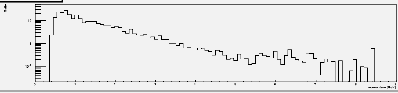
pi_yield/k_yield alpha=1.75
