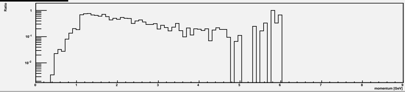
P_yield/k_yield alpha=11.75
