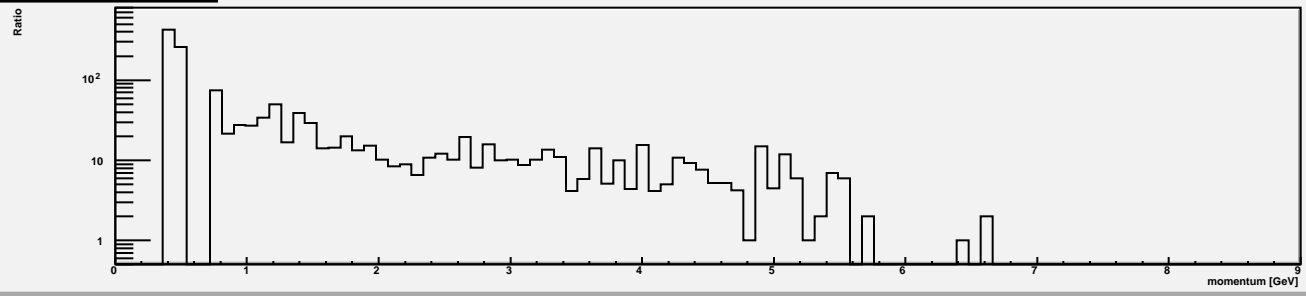
pi_yield/k_yield alpha=11.75
