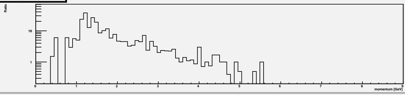
pi_yield/k_yield alpha=11.75
