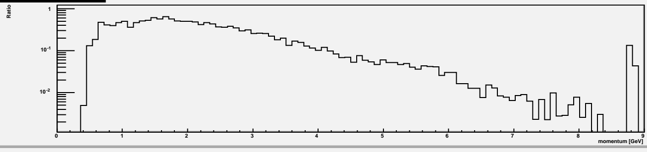
P_yield/k_yield alpha=2.75
