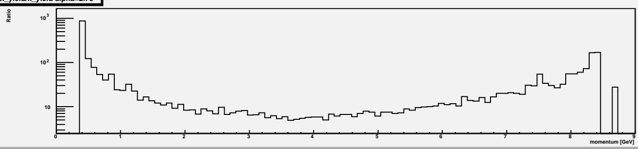
pi_yield/k_yield alpha=2.75
