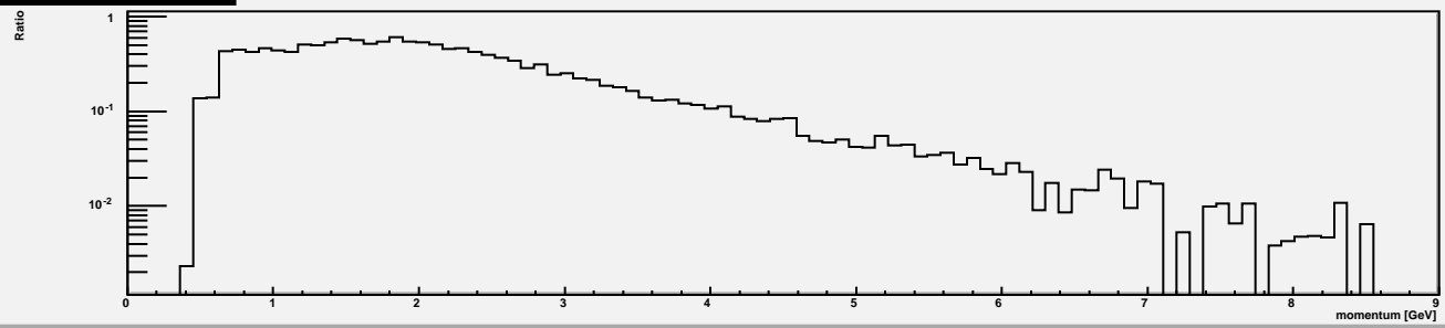
P_yield/k_yield alpha=3.75
