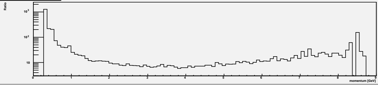
pi_yield/k_yield alpha=3.75
