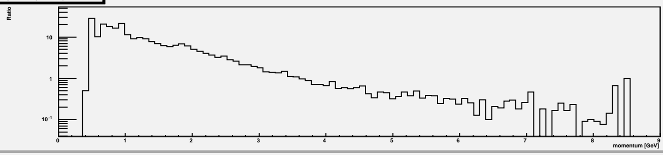
pi_yield/k_yield alpha=3.75
