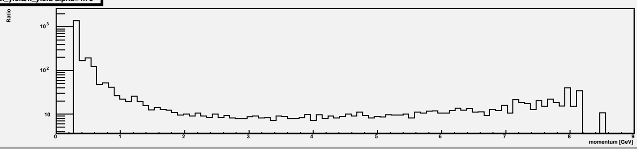
pi_yield/k_yield alpha=4.75
