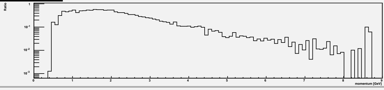
P_yield/k_yield alpha=4.75
