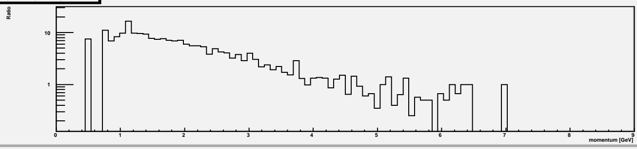
pi_yield/k_yield alpha=9.75
