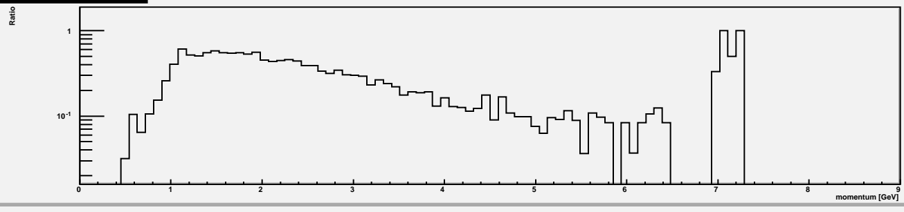
P_yield/k_yield alpha=9.75
