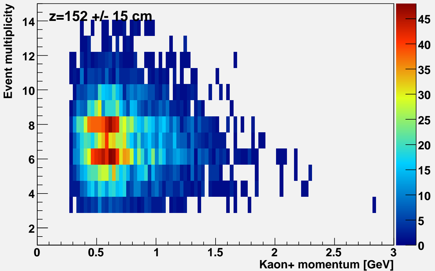
Event multiplicity vs k-momentum at bcal z=152
