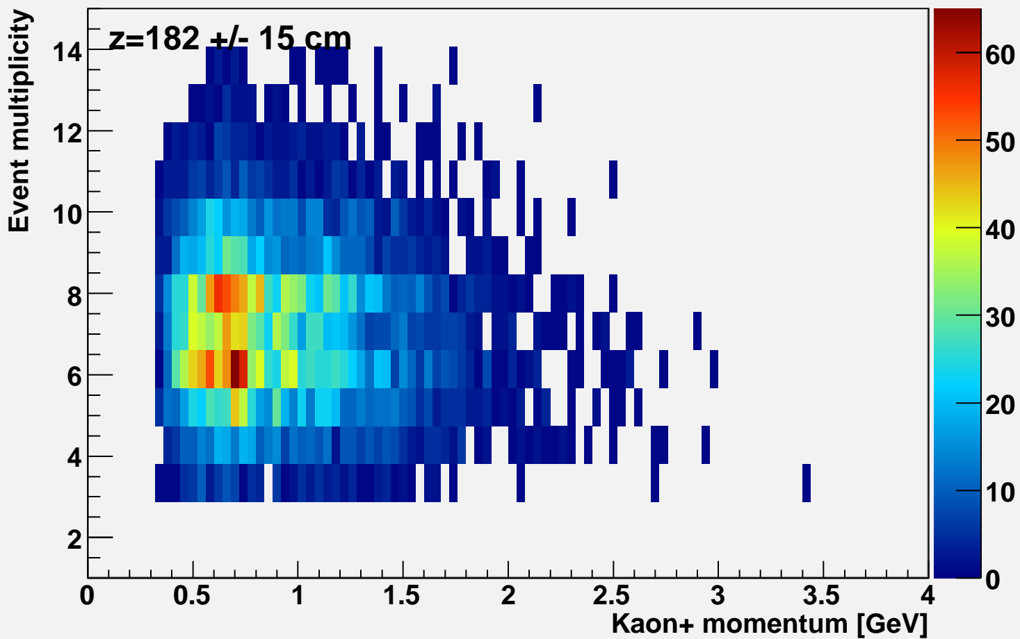
Event multiplicity vs k-momentum at bcal z=182
