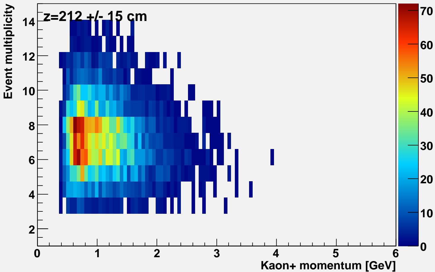
Event multiplicity vs k-momentum at bcal z=212
