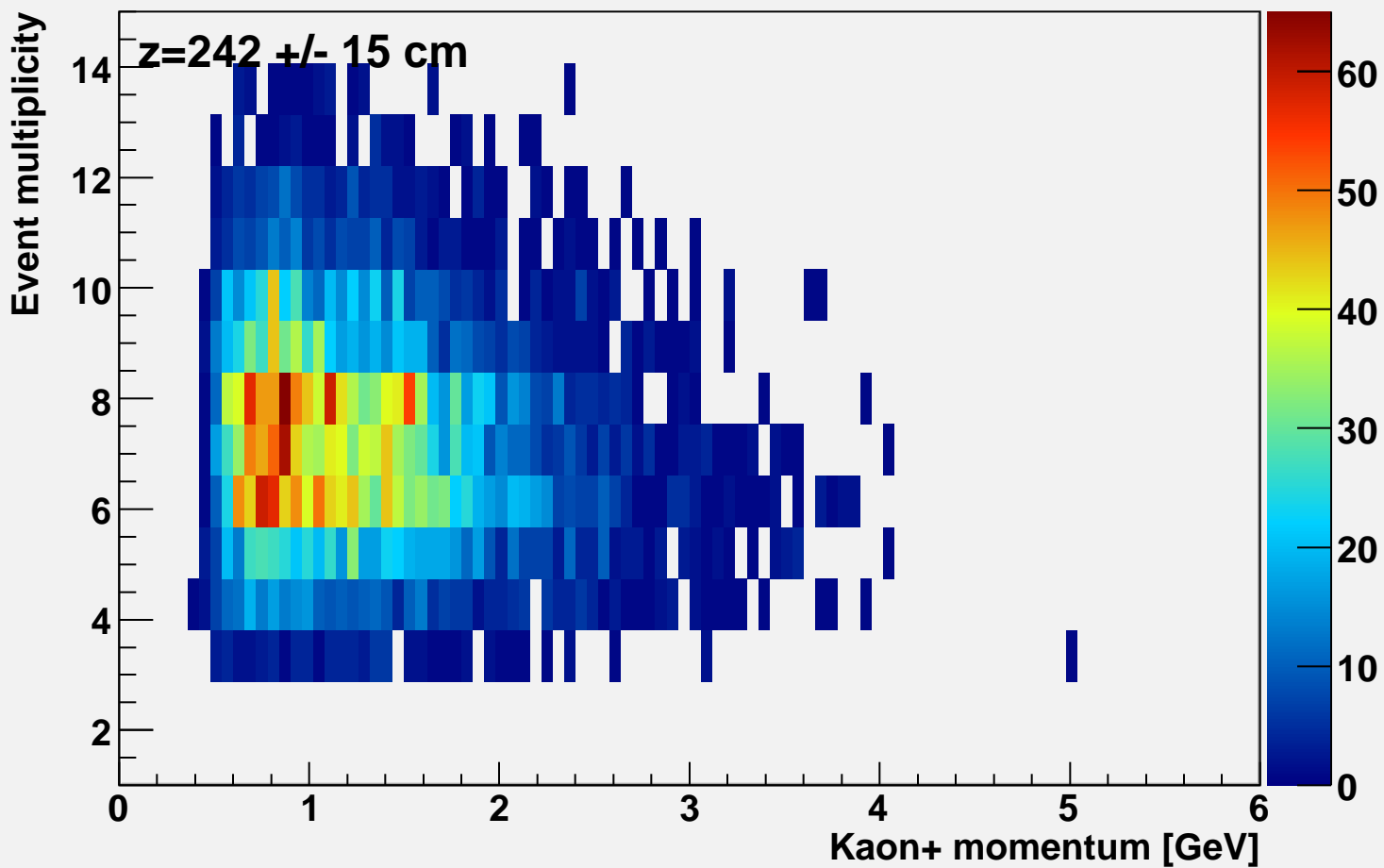
Event multiplicity vs k-momentum at bcal z=242
