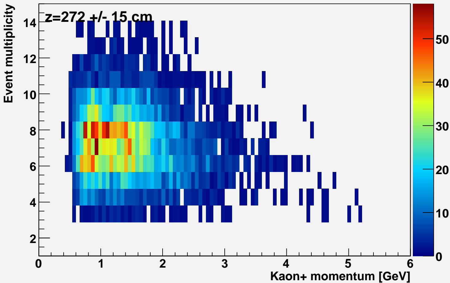
Event multiplicity vs k-momentum at bcal z=272
